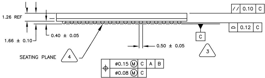
SIDE VIEW
