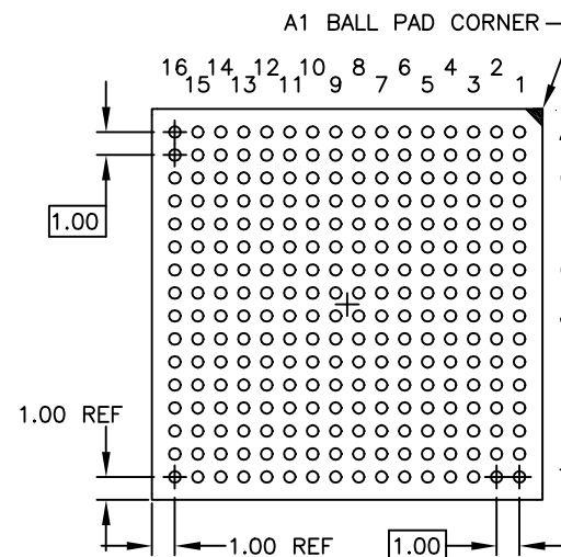
BOTTOM VIEW (BALL SIDE)
