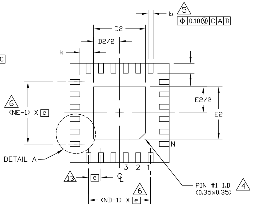
BOTTOM VIEW
