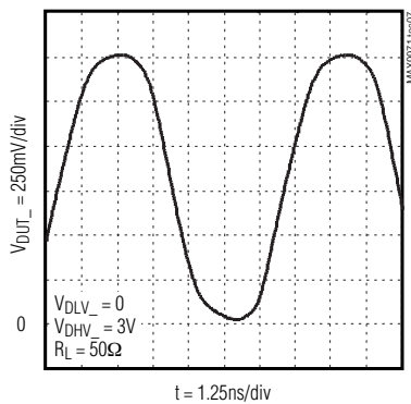
DRIVER 3Vp-p, 250Mbps SIGNAL RESPONSE
