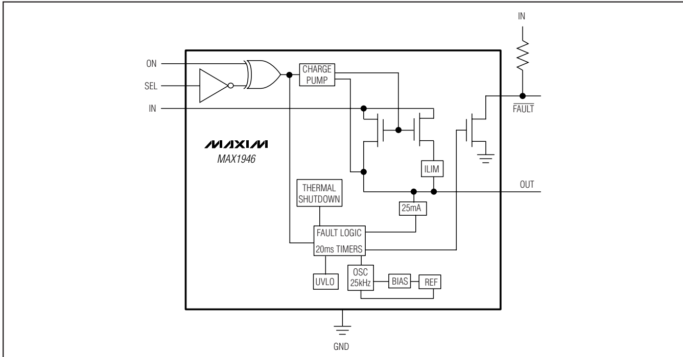
Figure 1. Functional Diagram
