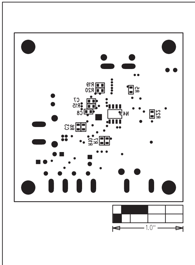
Figure 7. MAX17005D EV Kit Component Placement Guide—Solder Side
