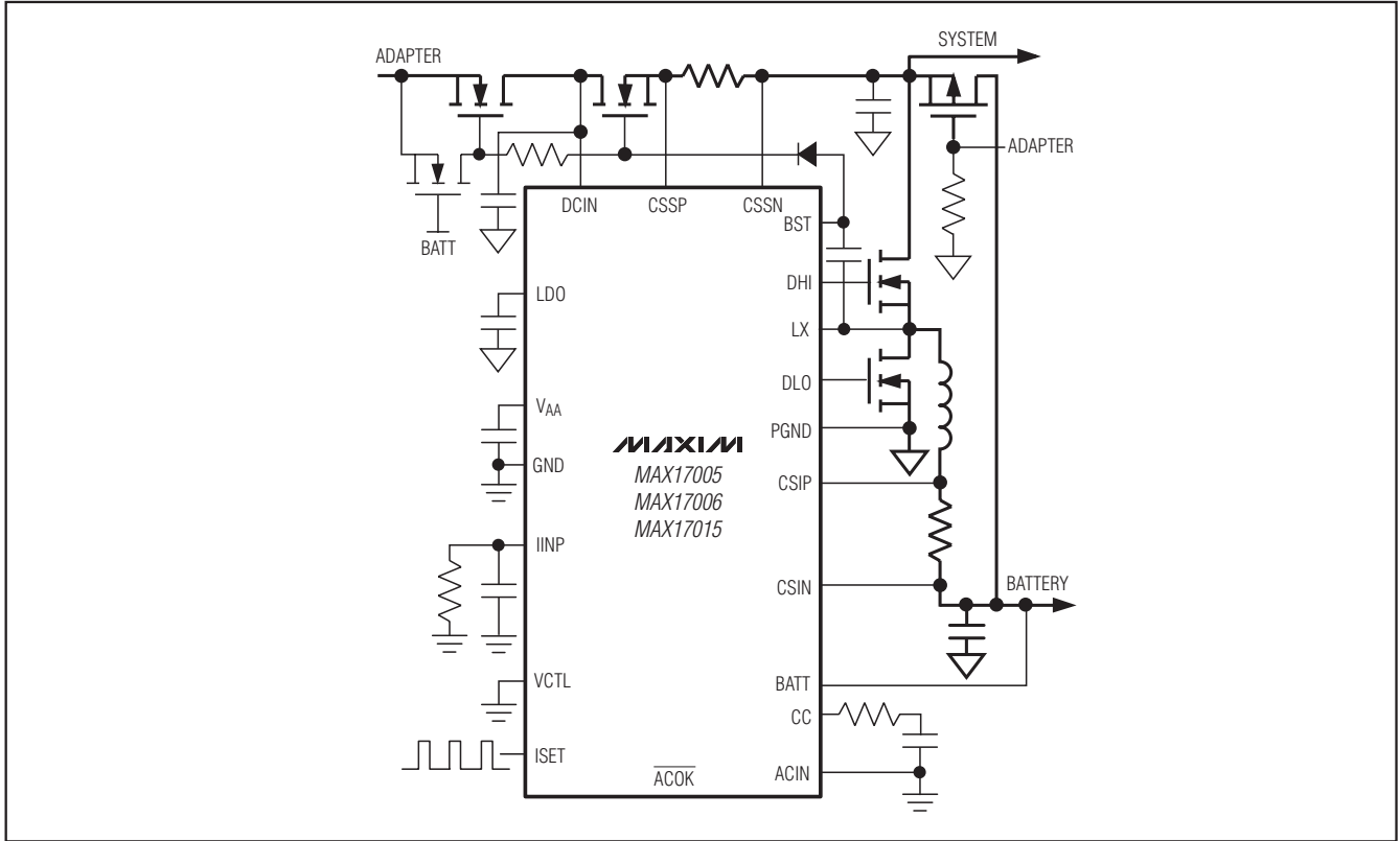
Minimal Operating Circuit
