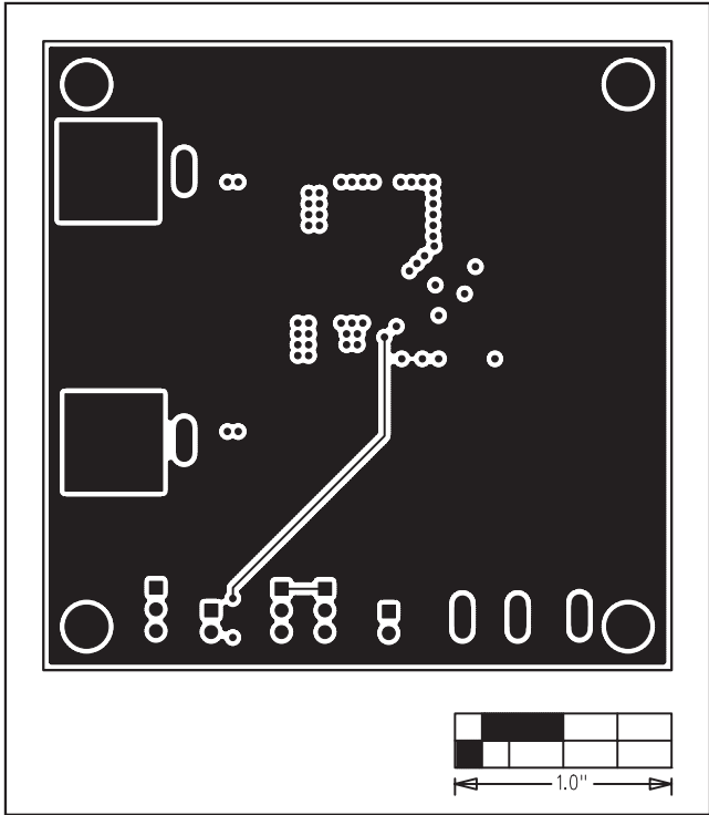
Figure 5. MAX15038 EV Kit PCB Layout—Layer 3
