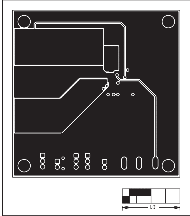
Figure 6. MAX15038 EV Kit PCB Layout—Solder Side
