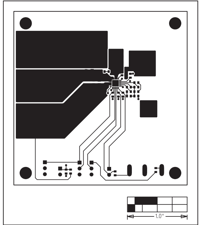
Figure 3. MAX15038 EV Kit PCB Layout—Component Side
