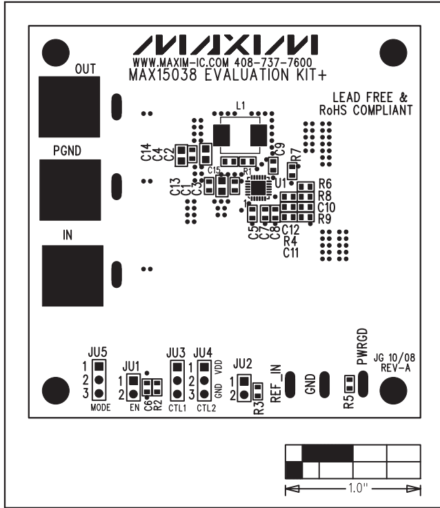
Figure 2. MAX15038 EV Kit Component Placement Guide—Component Side
