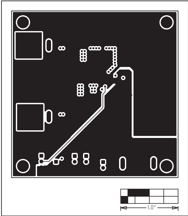
Figure 4. MAX15038 EV Kit PCB Layout—Layer 2
