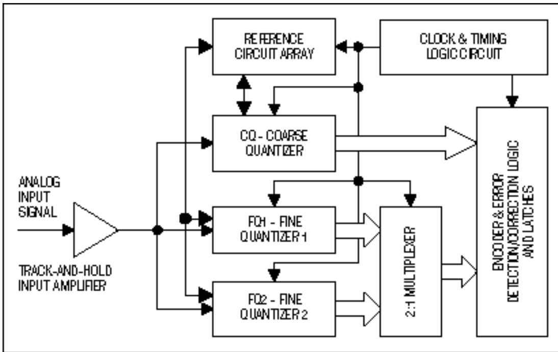
Figure 2. Principle of the time-interleaved two-step flash converter.
