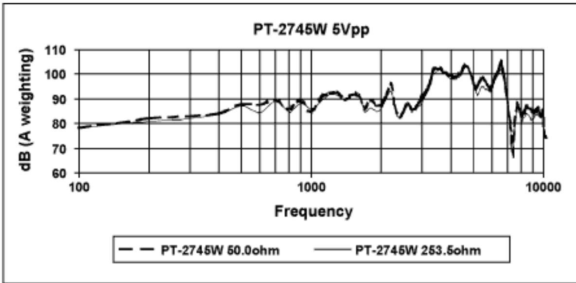
Figure 6. PT-2745W with 5Vpp excitation.
