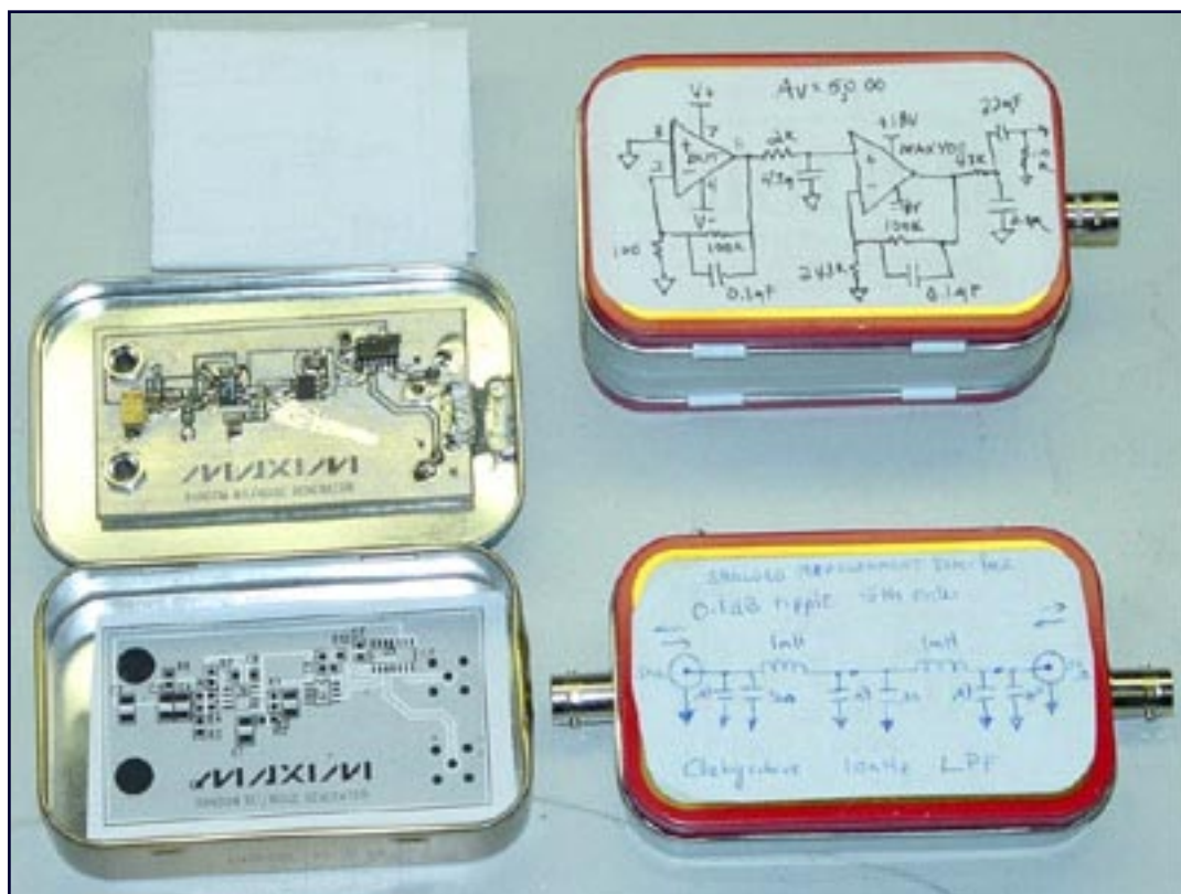
Figure 1. Disposable candy containers make excellent test fixture enclosures.
