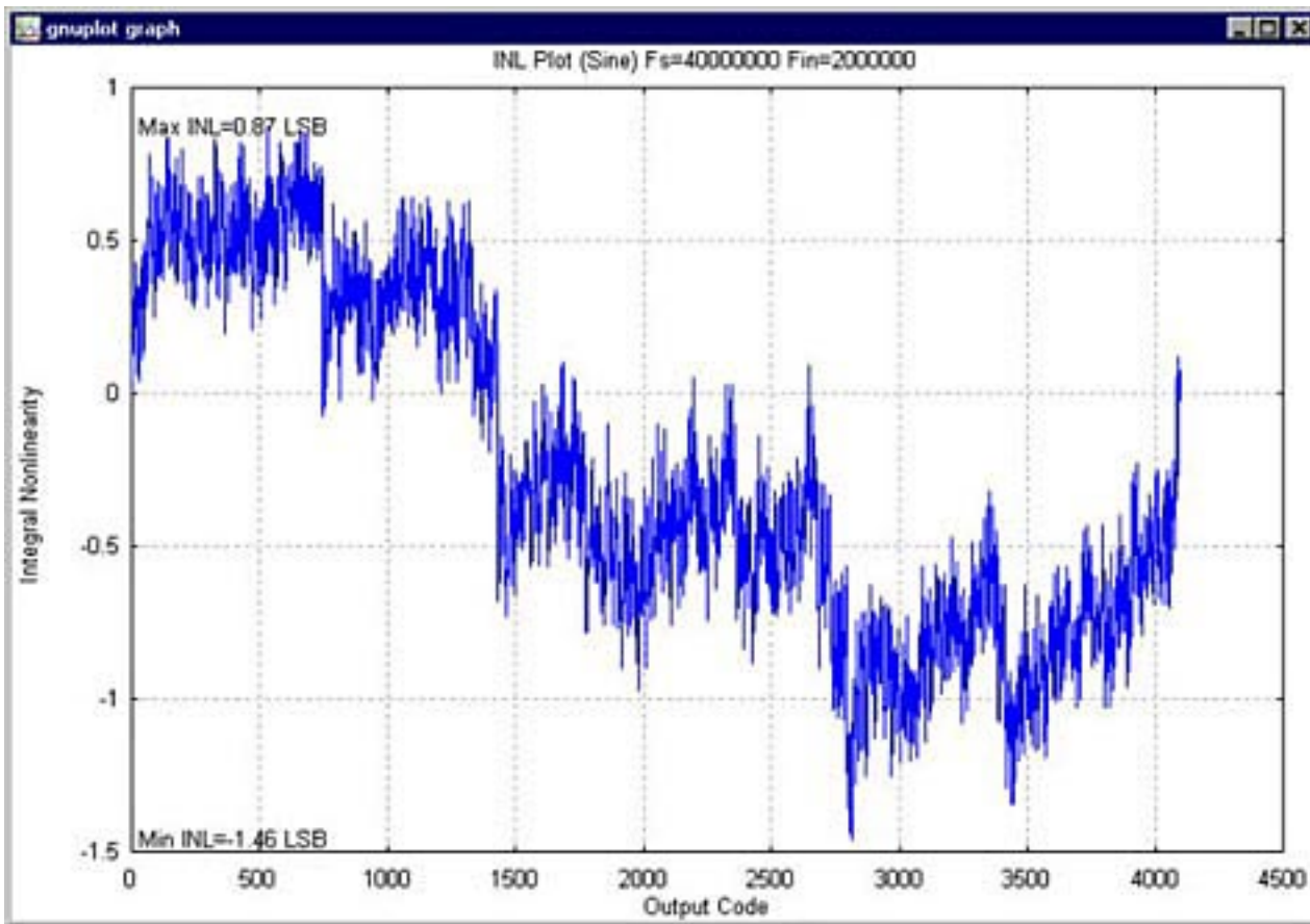
Figure 7. INL plot.
