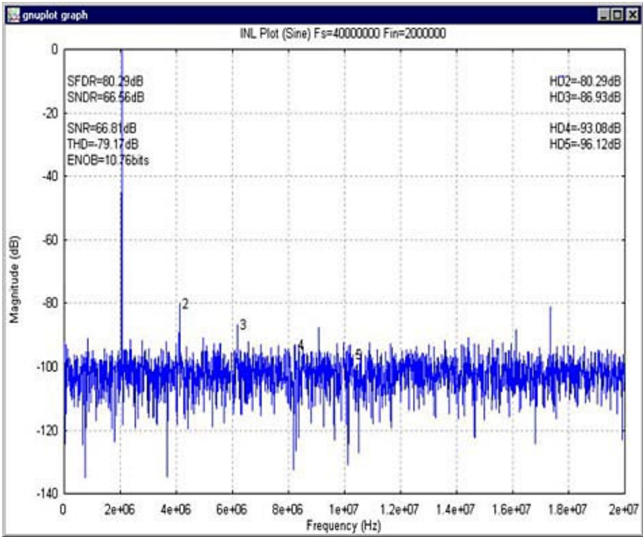
Figure 4. Dynamic performance (FFT) Plot.
