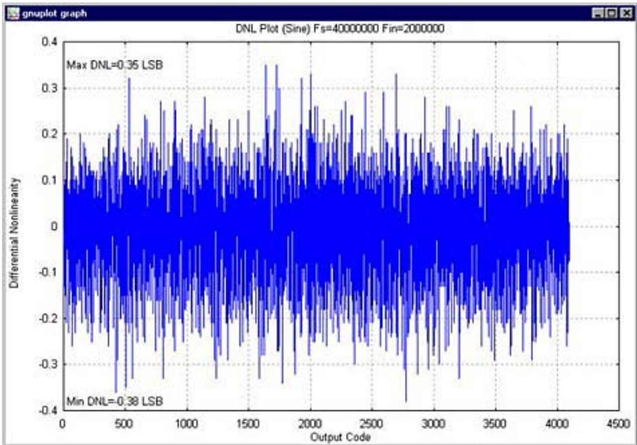
Figure 6. DNL plot.
