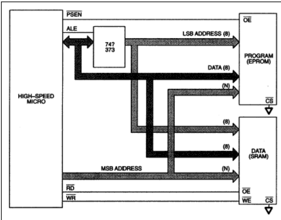
Figure 1. Typical high-speed micro system.
