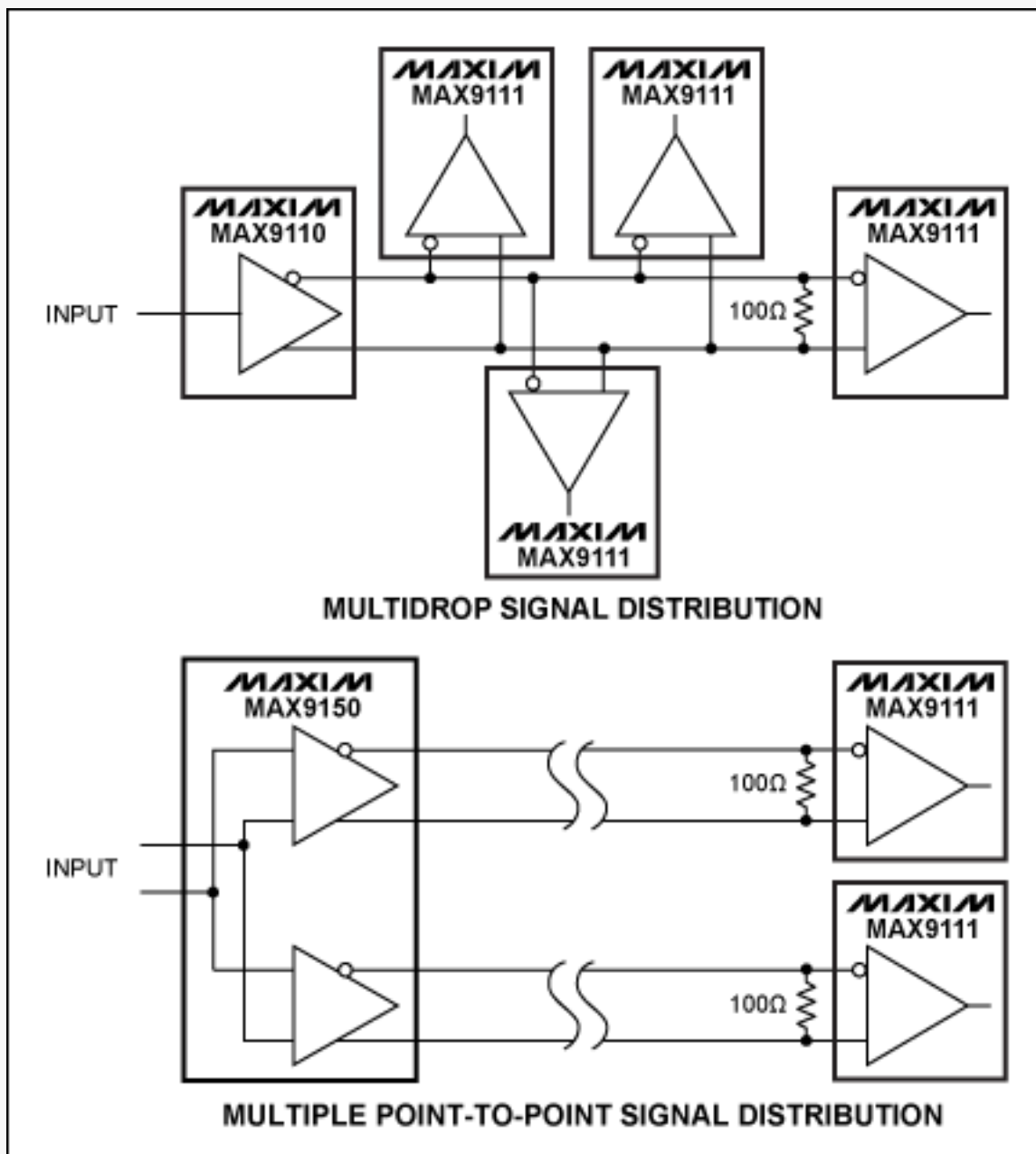
Figure 1. Multidrop signal distribution permits communication between one transmitter and multiple receivers. Multiple point-to-point signal distribution, which does not require tuning stubs, eliminates the disturbances that those stubs can potentially create.
