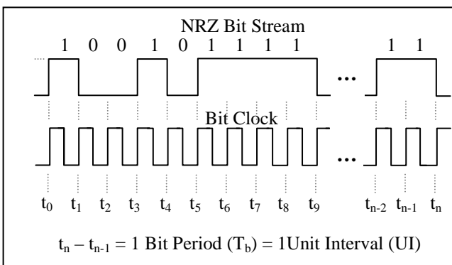
Figure 1. NRZ encoded bit stream
