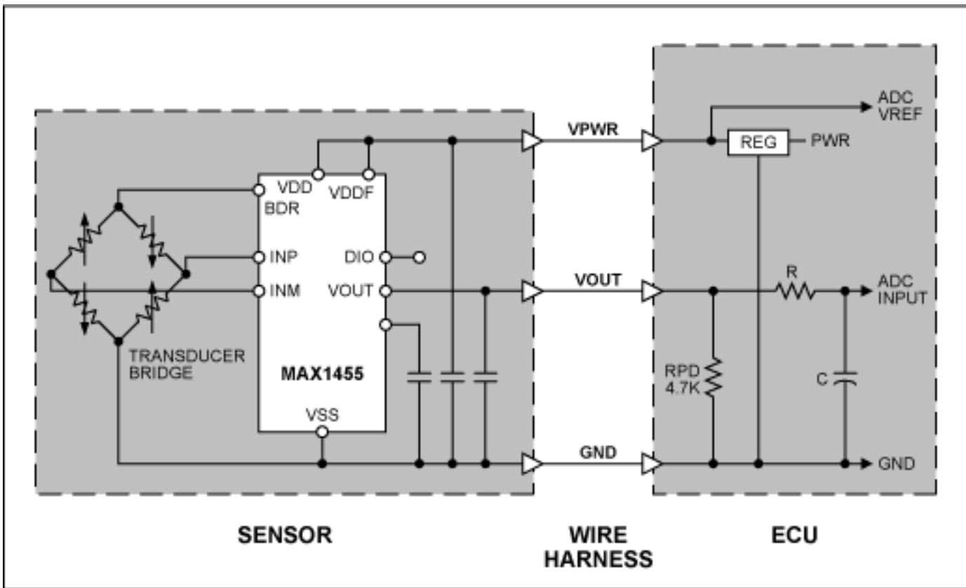
Figure 2. Typical sensor wiring configuration.
