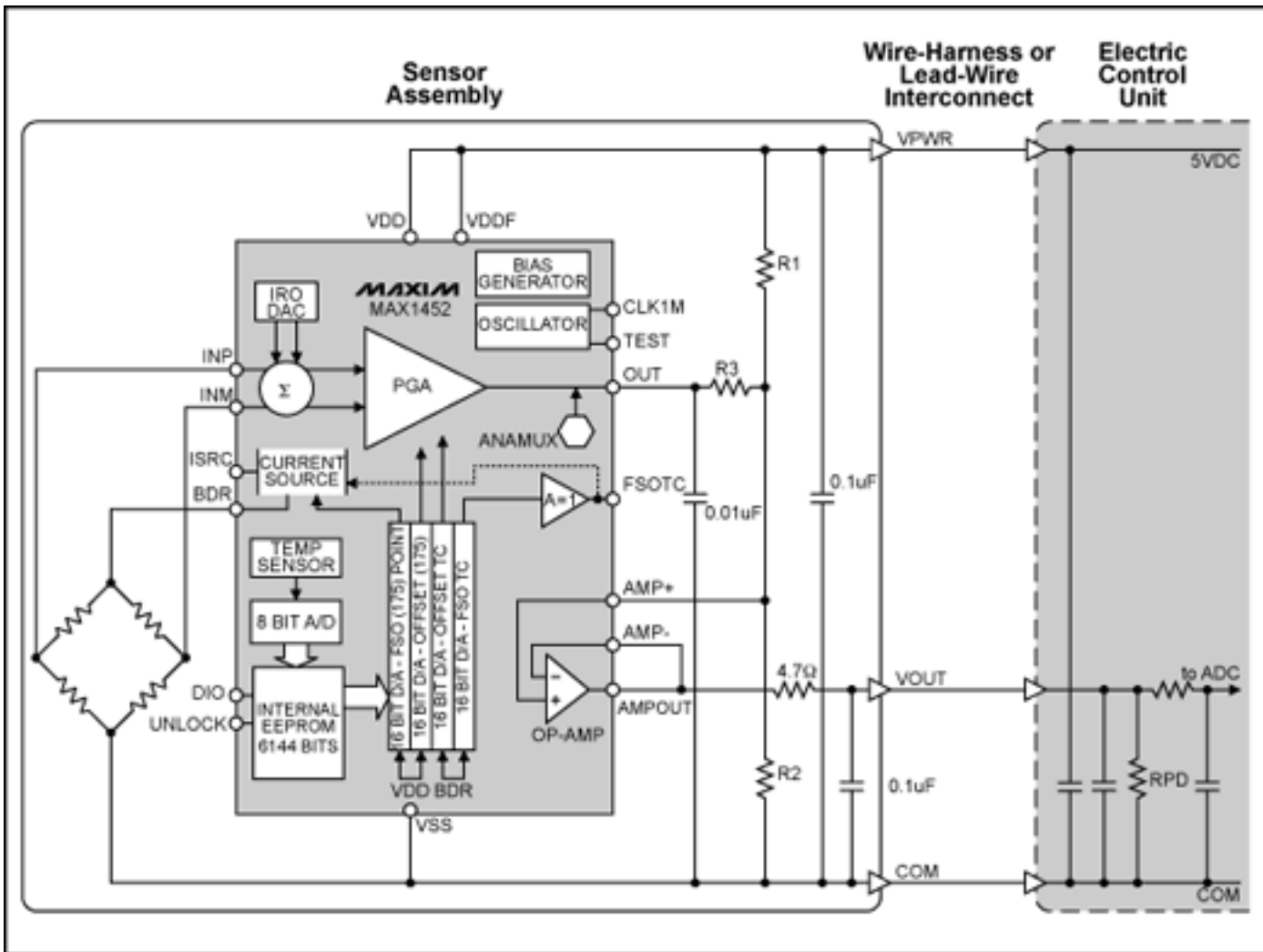
Figure 3. Typical sensor wiring configuration.
