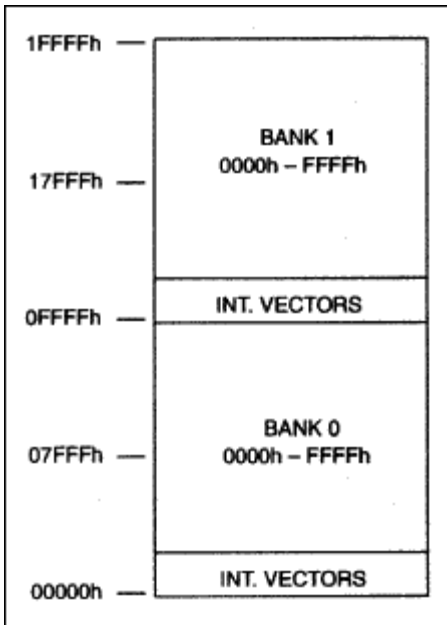
Figure 2. Simple page expansion example memory map.
