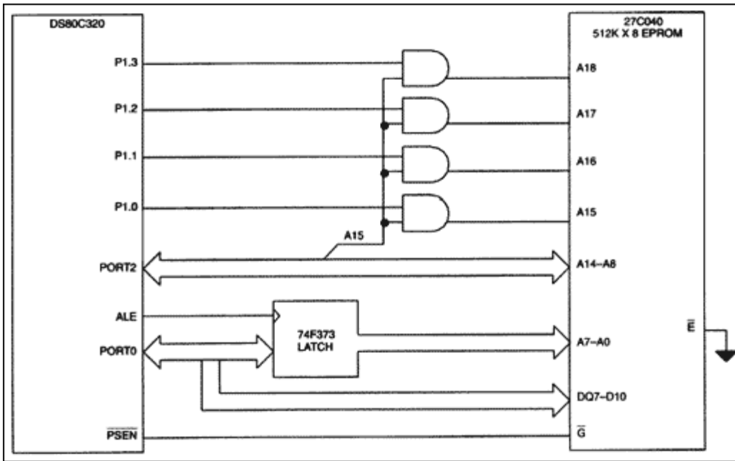
Figure 5. DS80C320 expanded memory example hardware configuration.
