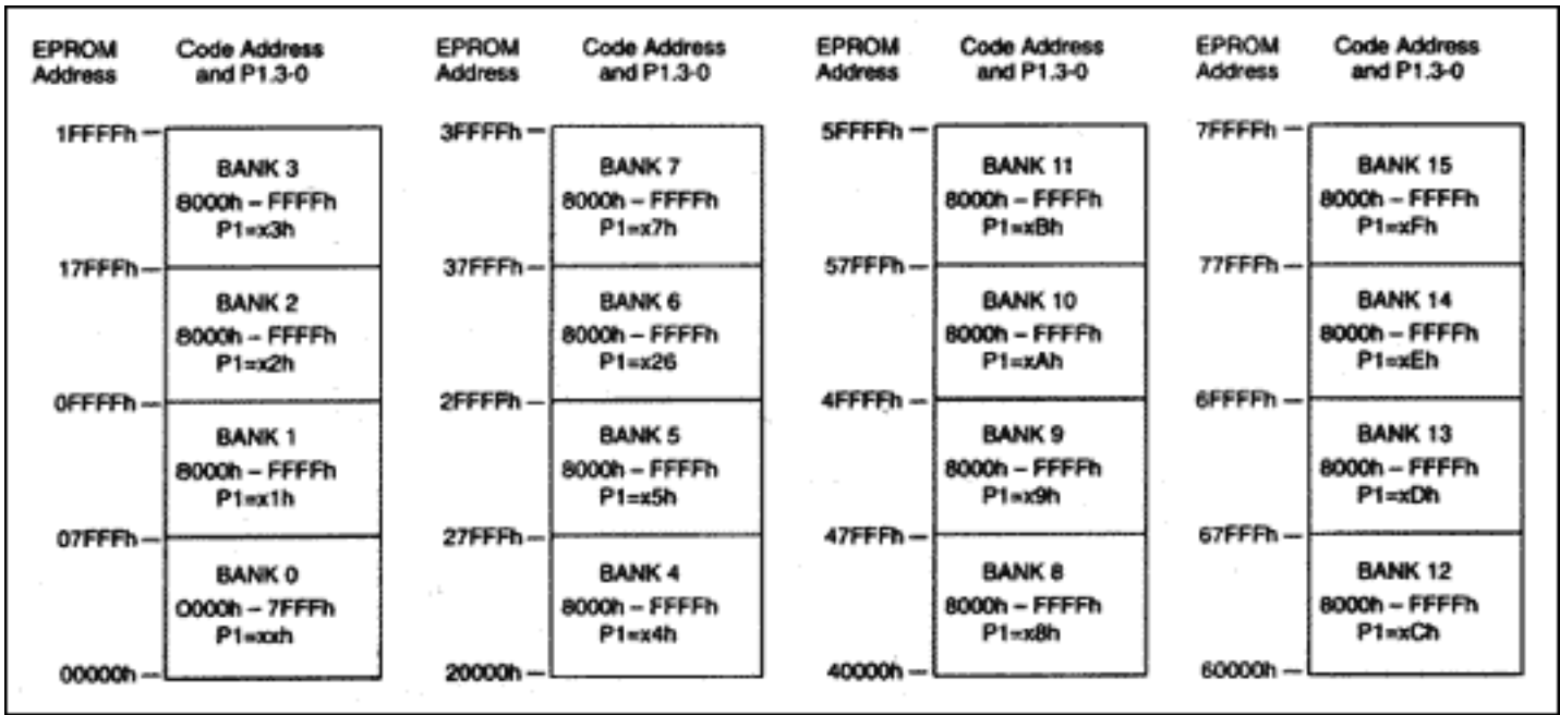
Figure 4. Common-page expansion memory example memory map.
