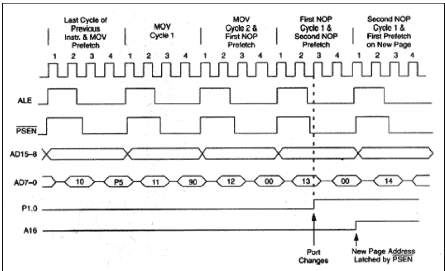
Figure 3. Bank switching timing diagram.
