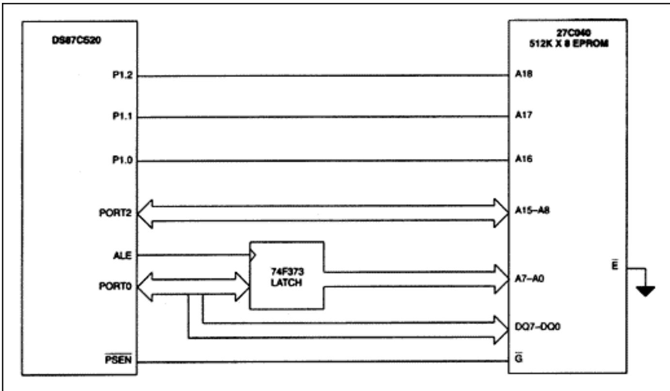
Figure 8. ROMSIZE Feature common-page I/O expansion.
