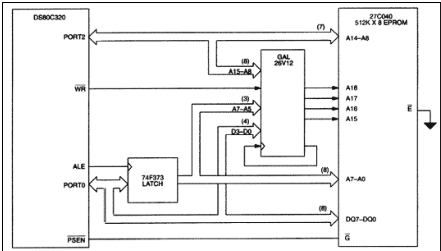
Figure 6. DS80C320 Latched address memory hardware example.
