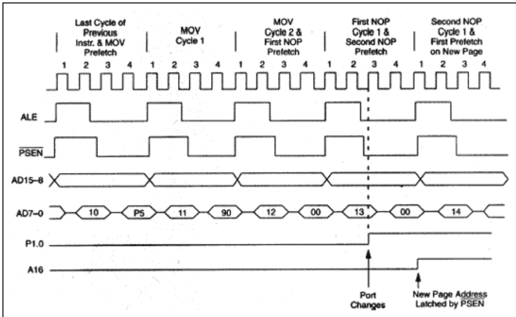
Figure 3. Bank switching timing diagram.
