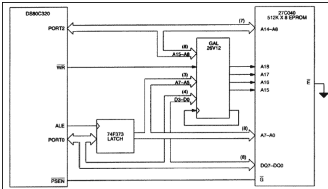
Figure 6. DS80C320 Latched address memory hardware example.
