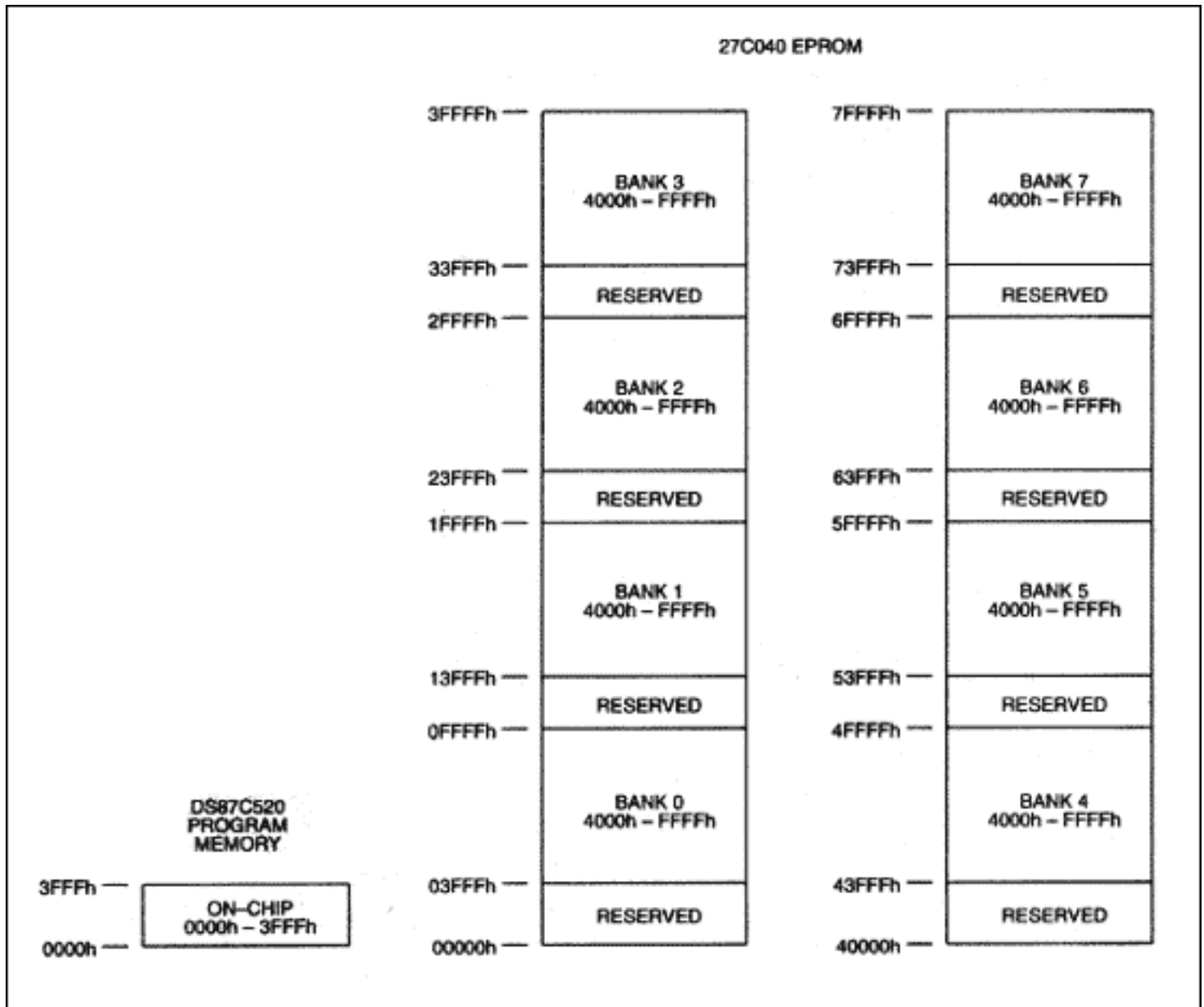
Figure 7. ROMSIZE Feature common-page expansion memory map.
