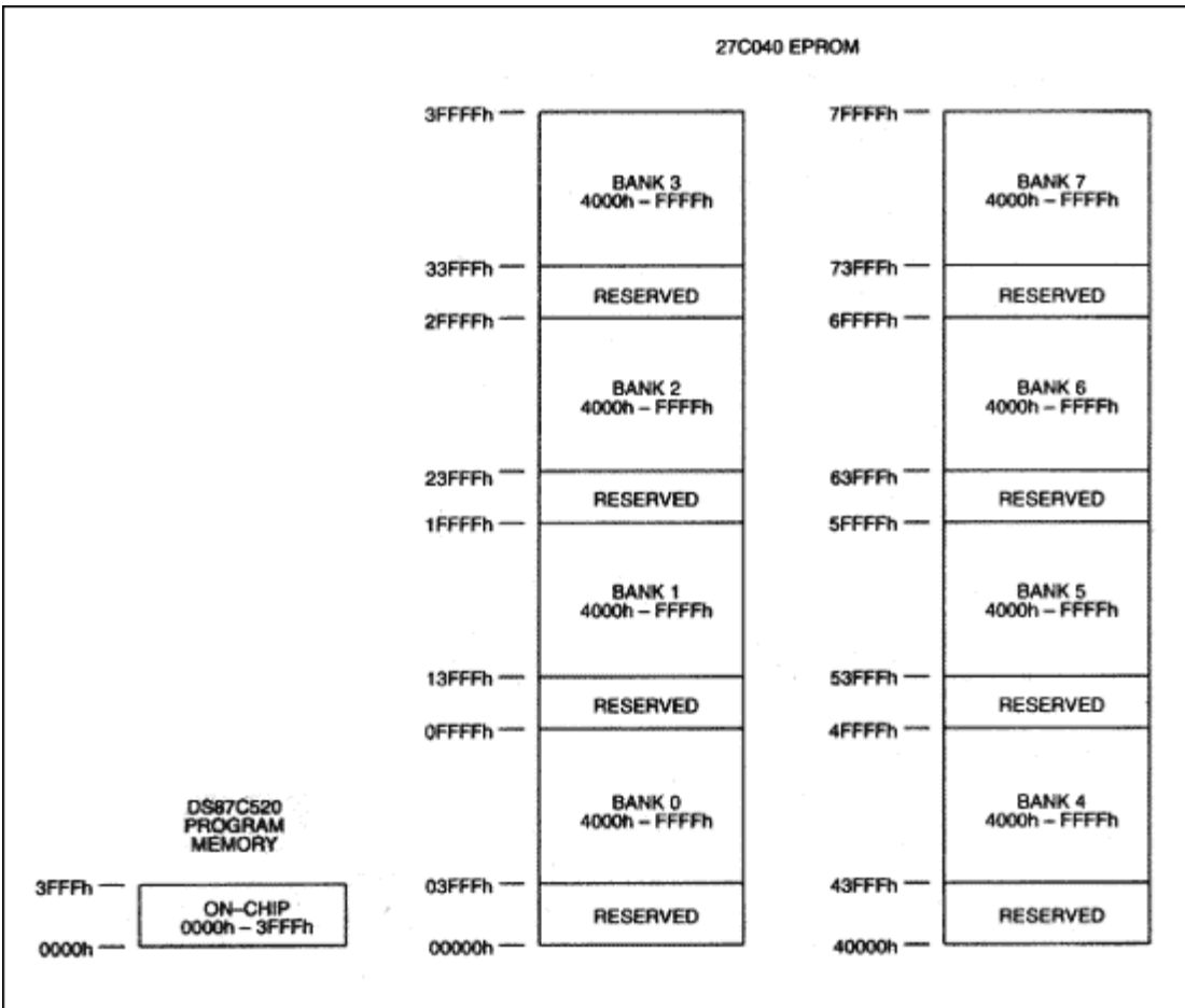
Figure 7. ROMSIZE Feature common-page expansion memory map.
