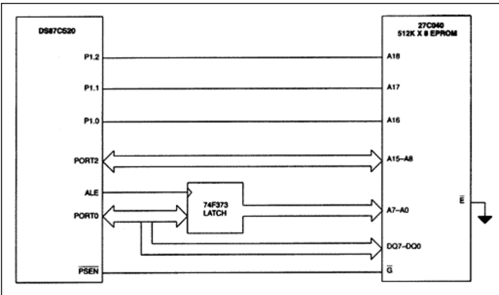
Figure 8. ROMSIZE Feature common-page I/O expansion.
