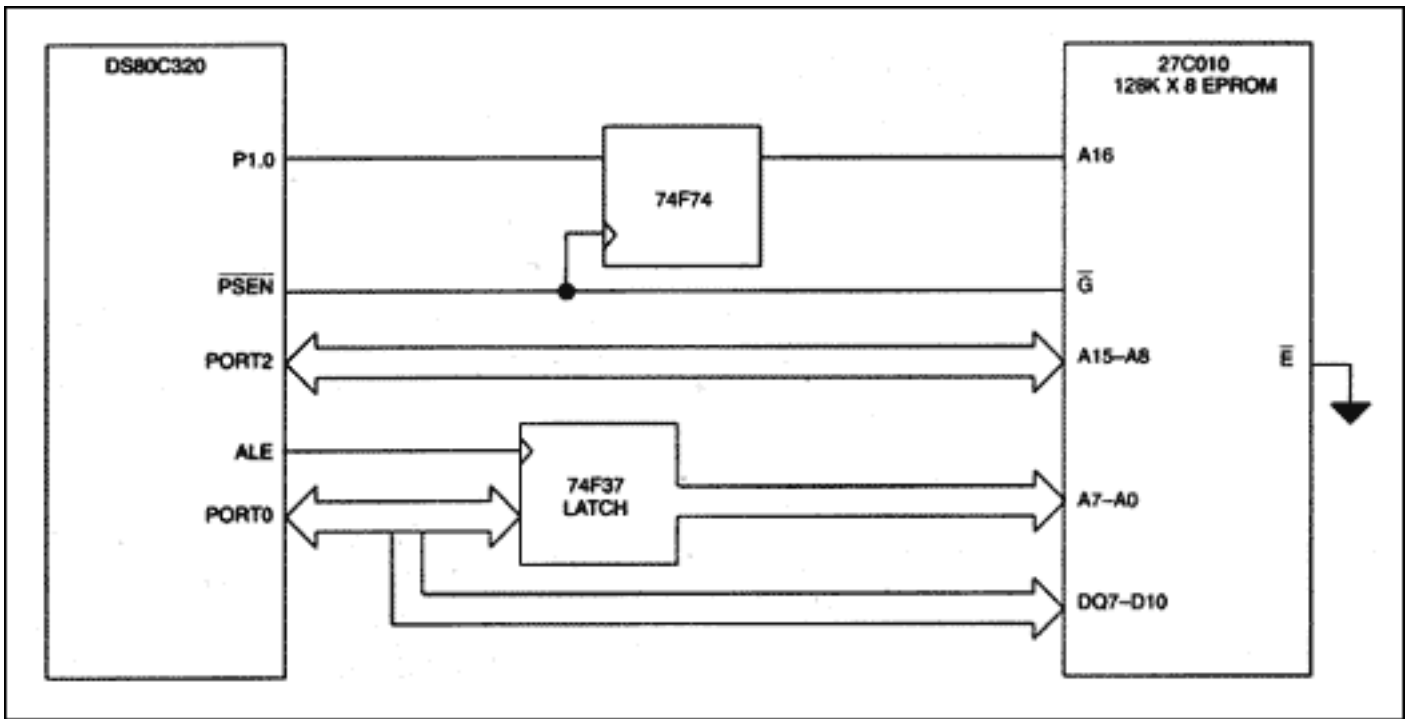
Figure 1. Simple page expansion example hardware.
