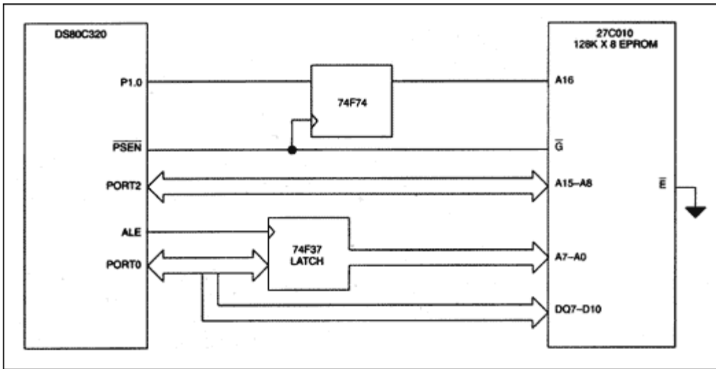
Figure 1. Simple page expansion example hardware.
