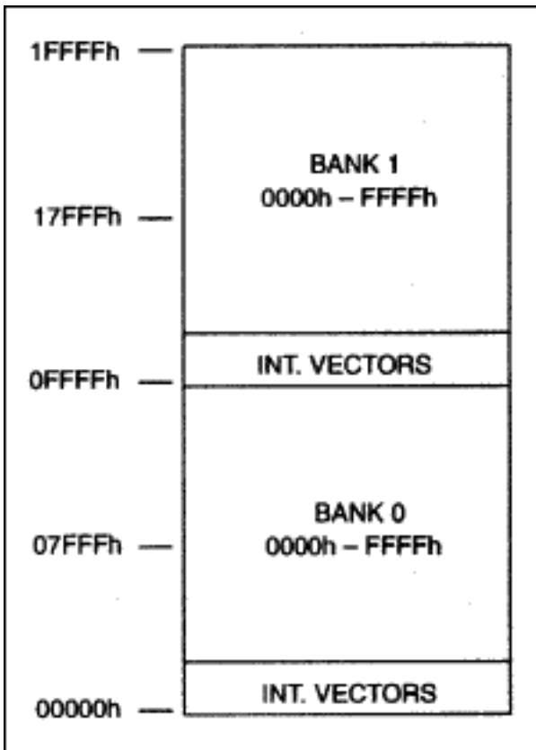
Figure 2. Simple page expansion example memory map.
