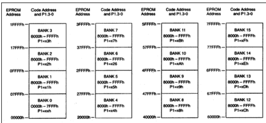
Figure 4. Common-page expansion memory example memory map.
