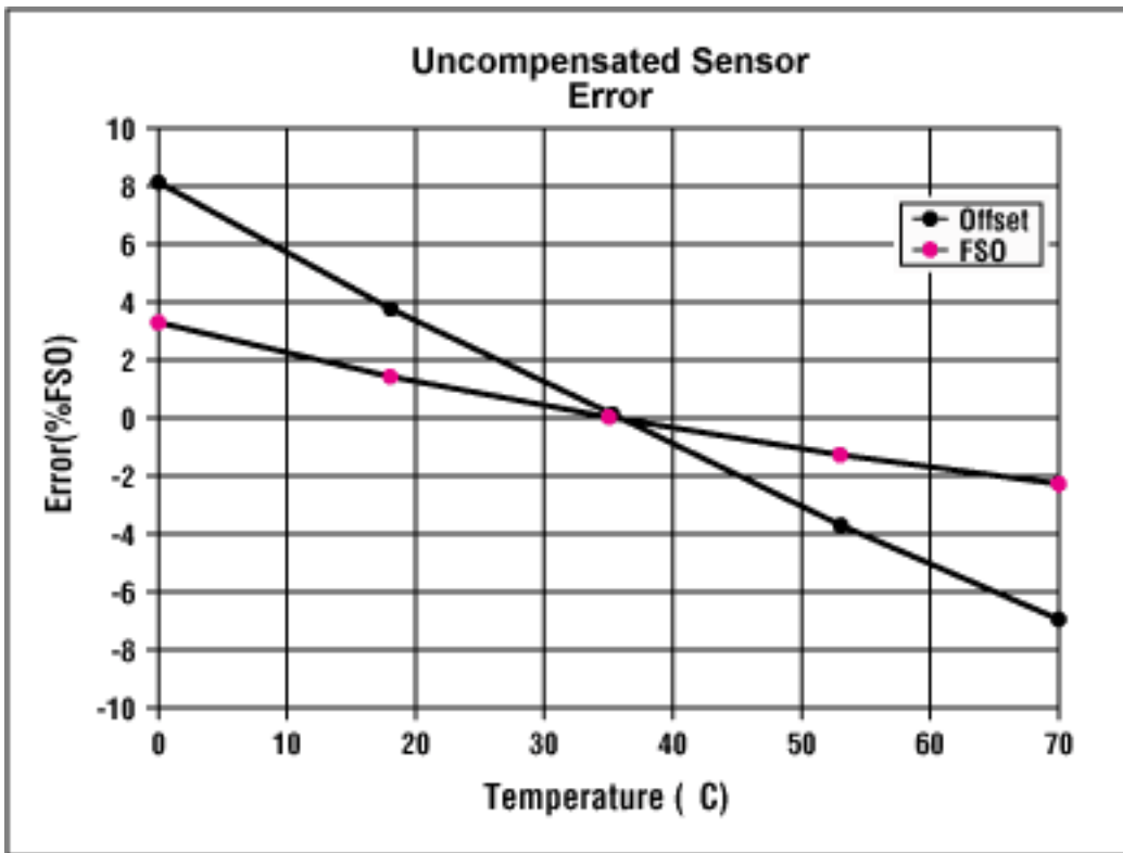
Figure 2. A slight curvature indicates second-order effects in the output of this piezoresistive transducer.
