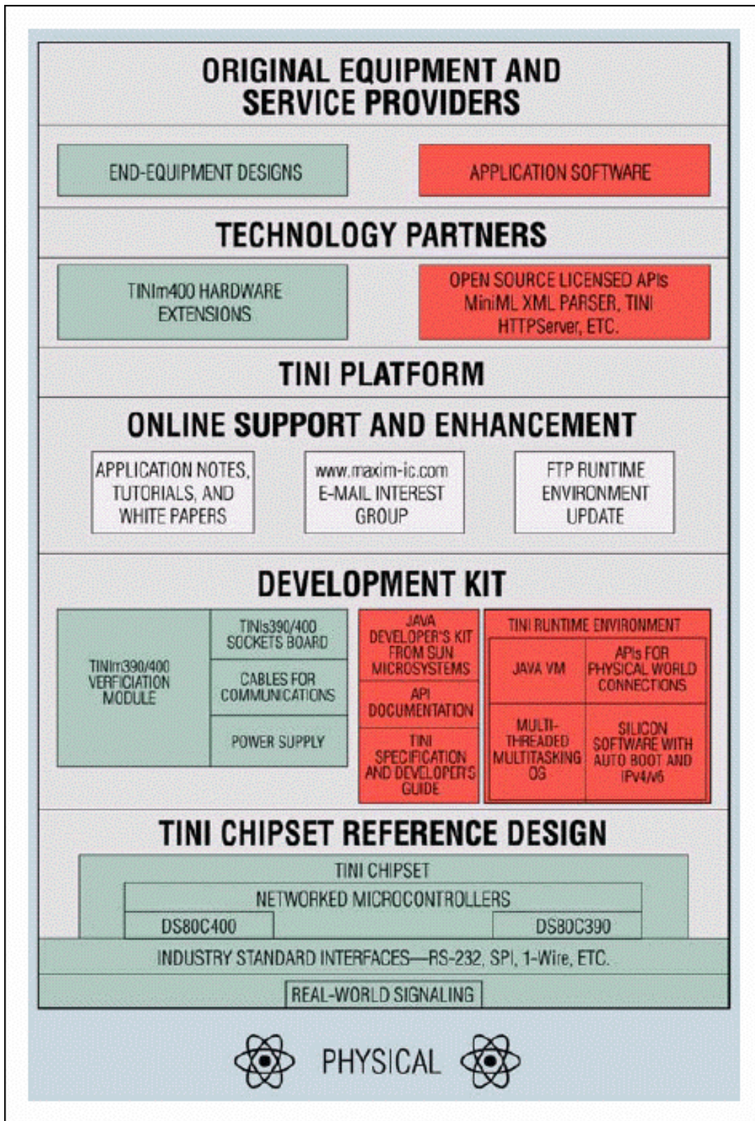
Figure 1. The TINI platform allow rapid prototyping and deployment of IP network-enabled real-world measurement.
