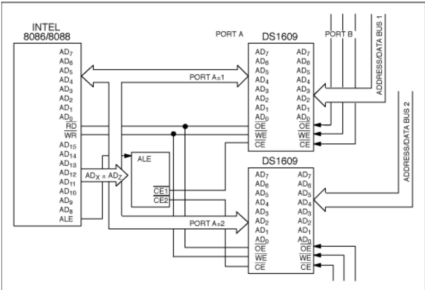
Figure 3. Multiplexed interface.
