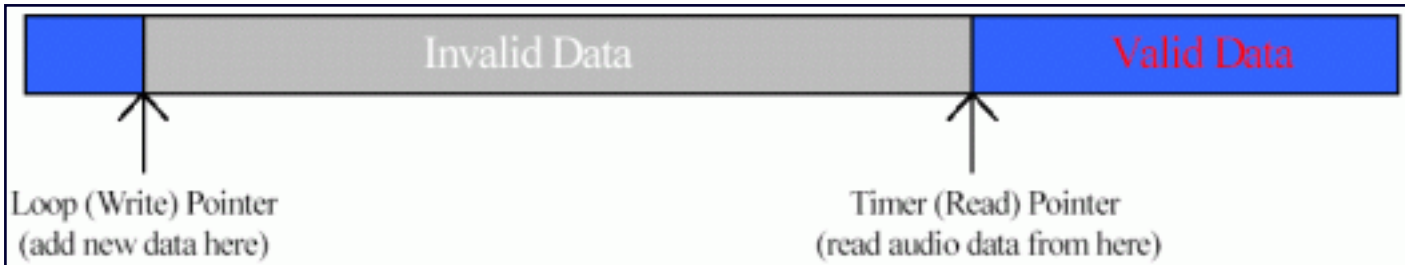
Figure 2. Circular audio buffer.
