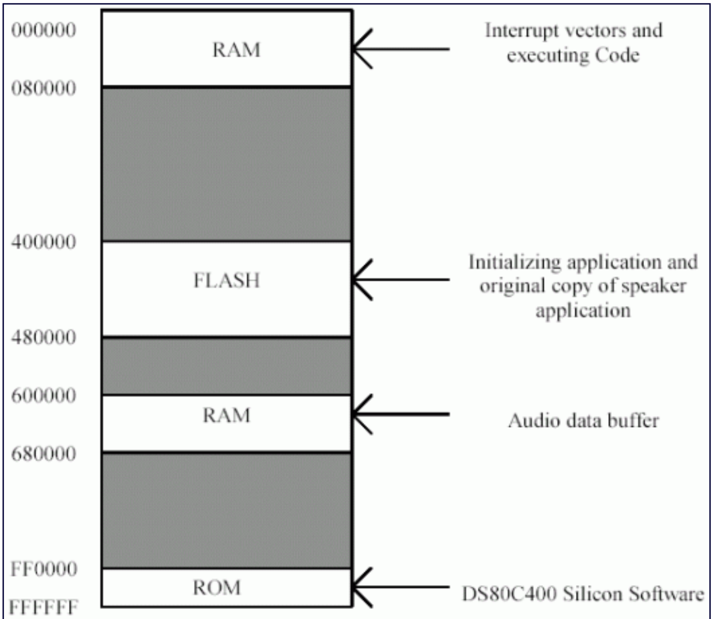
Figure 4. Board memory configuration.
