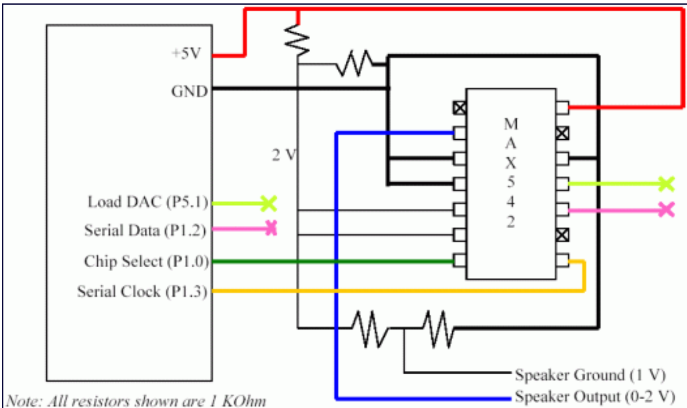
Figure 3. Hardware block diagram.
