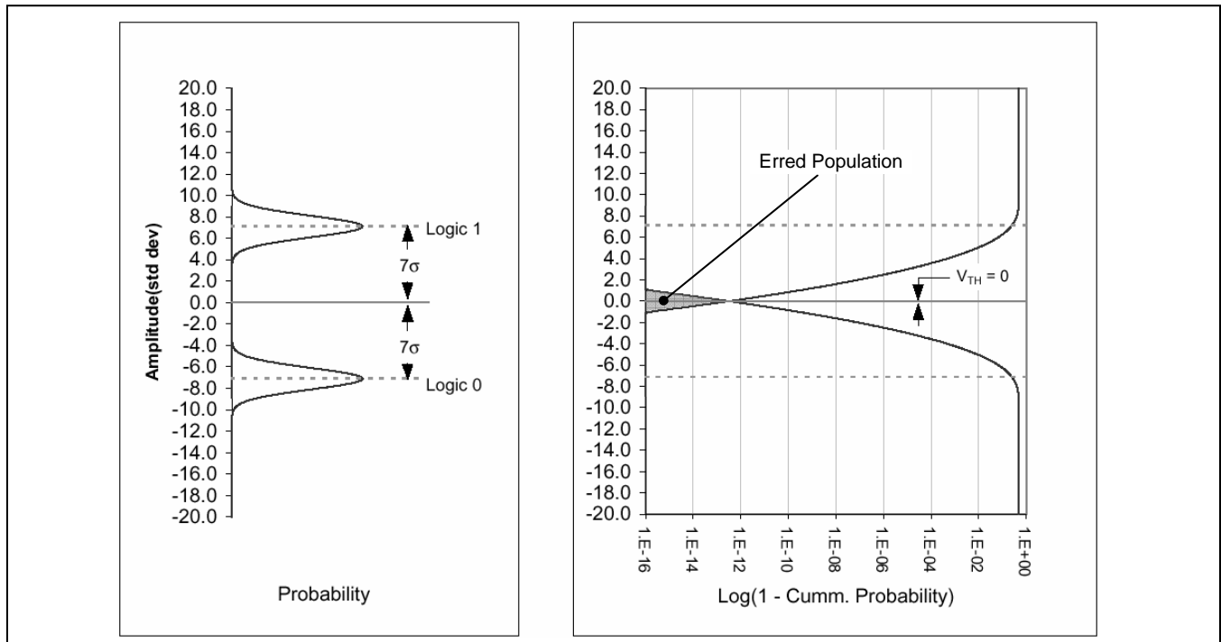
Figure 2. Noise distribution, as viewed linearly at the left, exhibits the familiar Gaussian distribution. Plotting the log(1-cummulative probability), at the right, reveals where the erred population is near the desired BER. With the decision threshold ( V_{TH} ) of 0V, a BER < 10^{-12} is theoretically possible.
