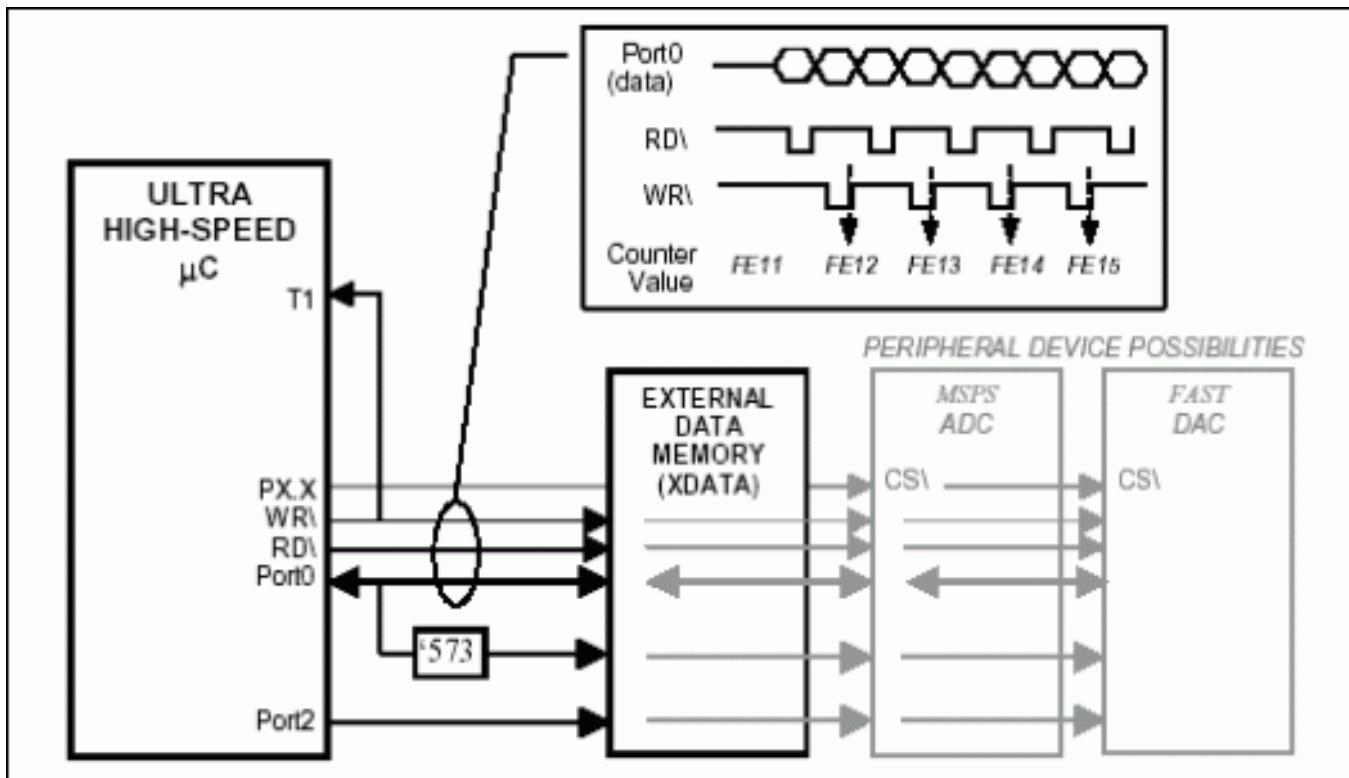
Figure 1. Hardware diagram for active-low wr strobe counting.
