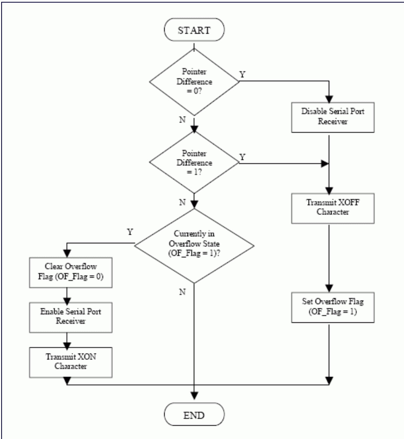
Figure 1. Overflow Handler Flowchart.
