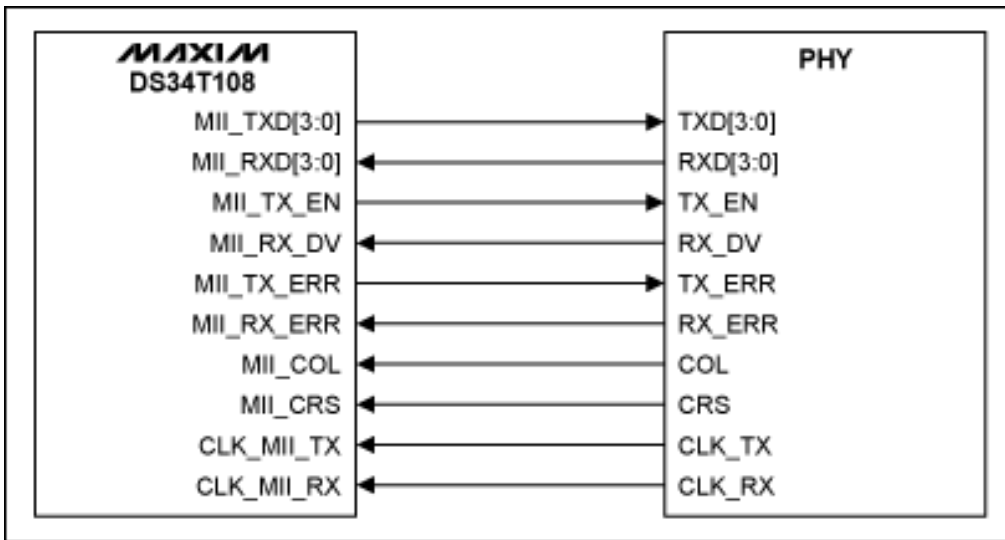
Figure 1. The DS34T108 is connected to an Ethernet PHY in MII mode.
