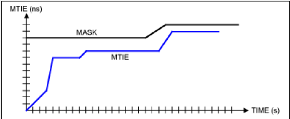
Figure 6. Typical MTIE graph with an MTIE mask.
