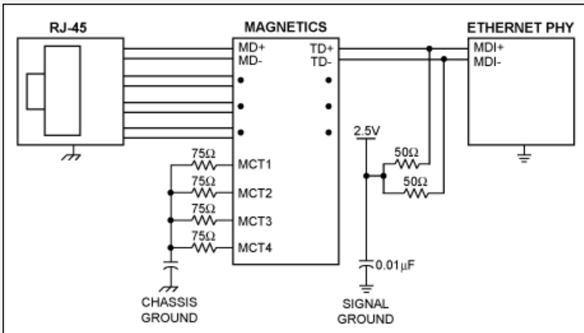
Figure 3. Typical Ethernet PHY connection.
