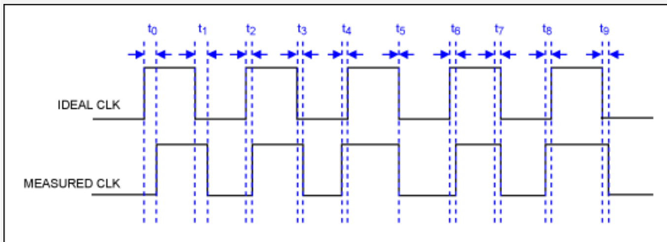
Figure 4. TIE measurement against an ideal source.
