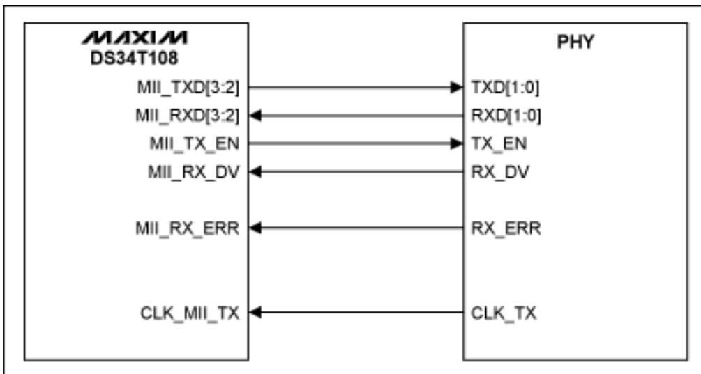
Figure 2. The DS34T108 is connected to an Ethernet PHY in RMII mode.
