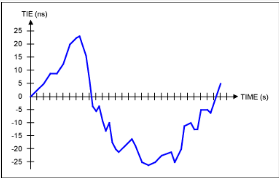
Figure 5. Typical TIE plotted over time.
