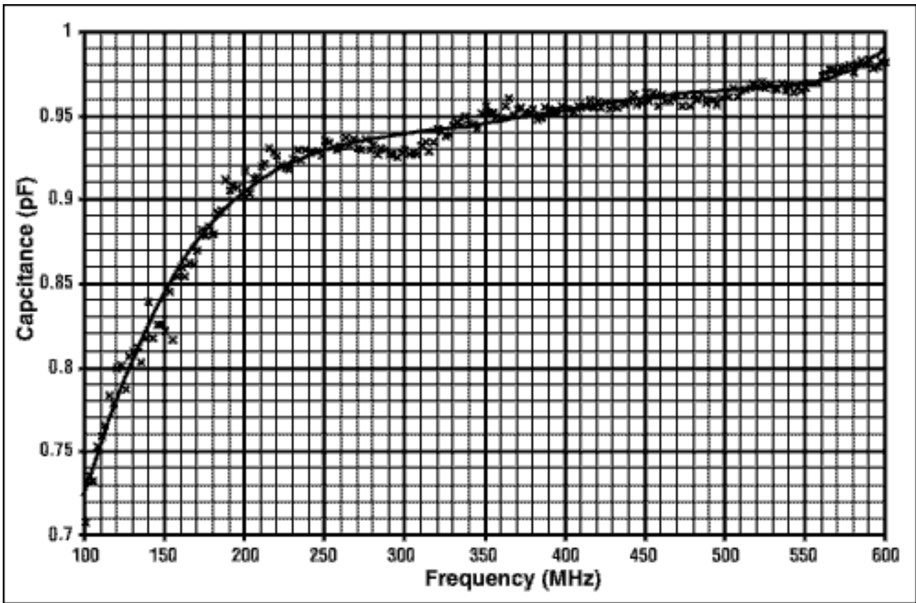
Figure 11. C_{int} vs. frequency for the MAX2310 high-band tank (sixth-order polynomial curve fit)
