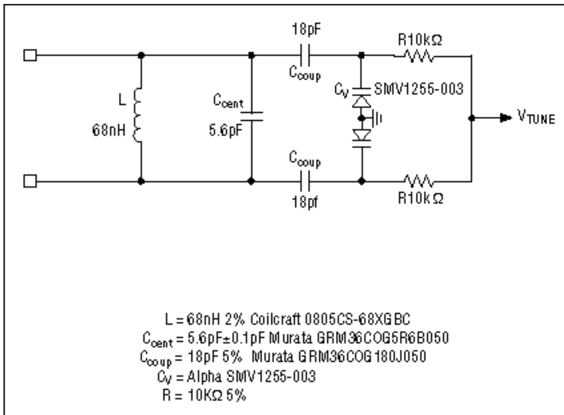
Figure 6. 85MHz low-band IF tank schematic.
