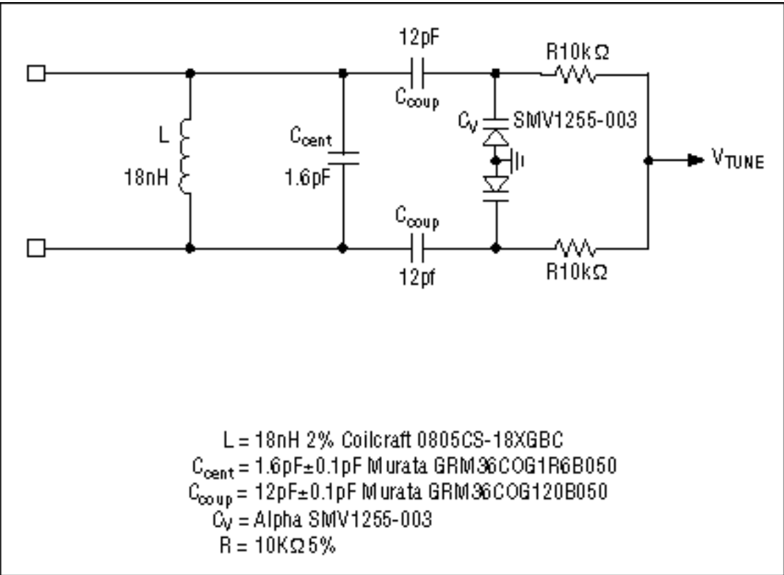
Figure 8. 210MHz high-band IF tank schematic.
