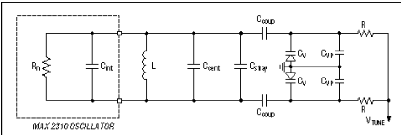
Figure 3. Lumped C stray model.
