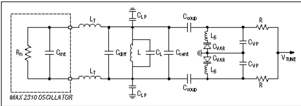
Figure 4. Detailed VCO model.
