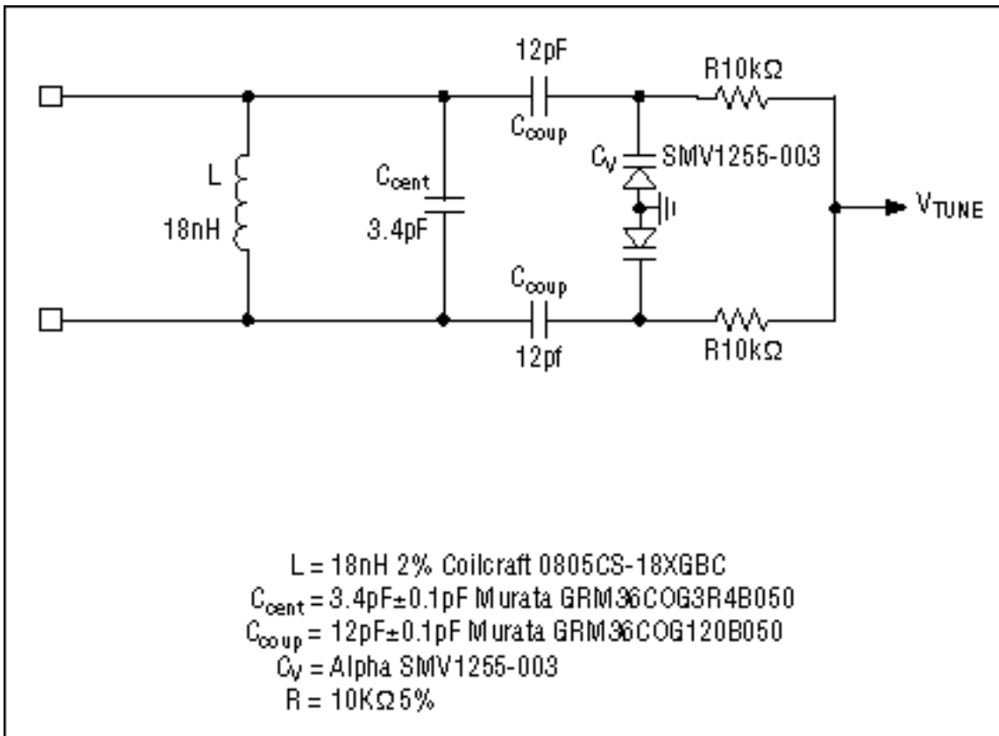
Figure 7. 190MHz high-band IF tank schematic.
