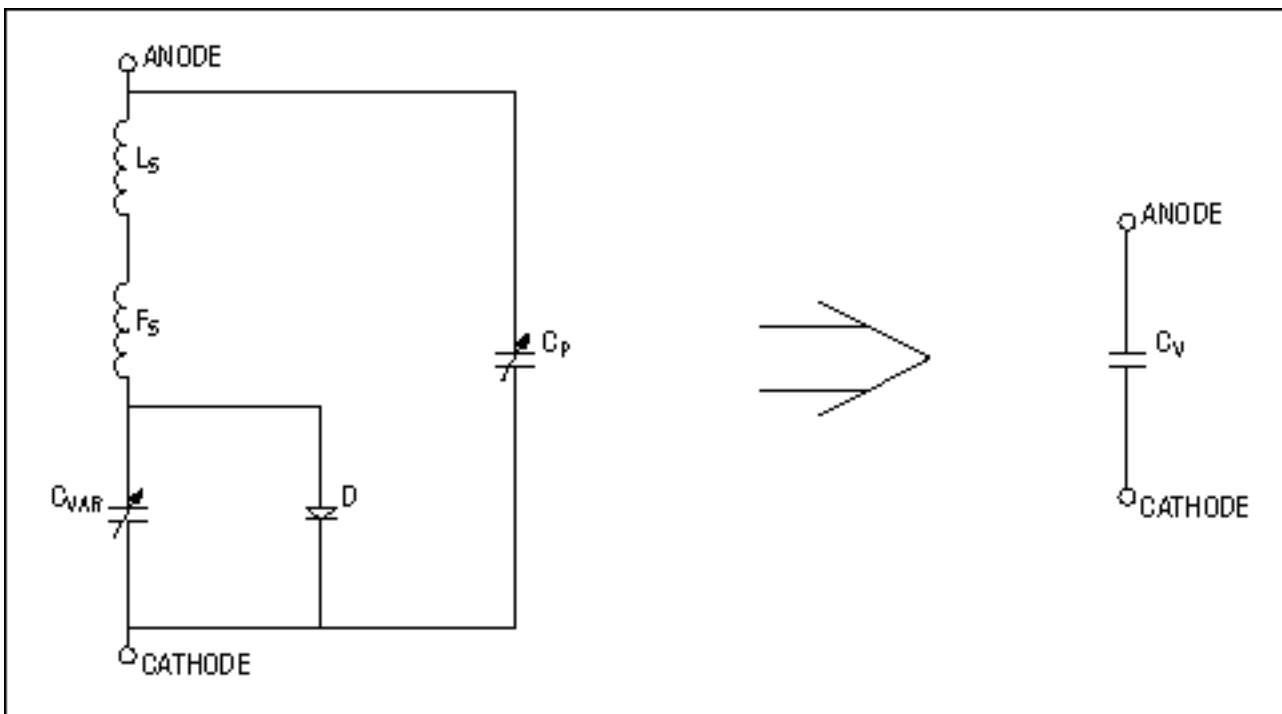
Figure 10. Varactor model.
