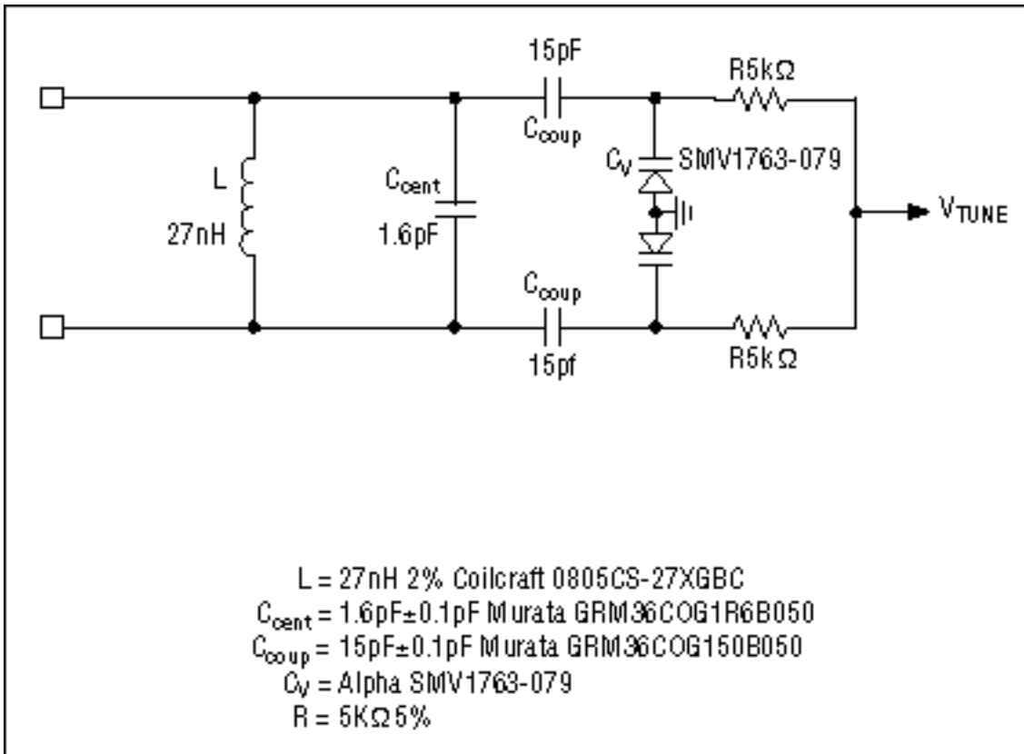
Figure 9. High-Q 210MHz high-band IF tank schematic.
