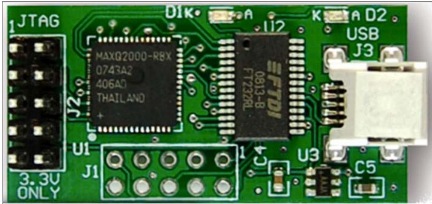
Figure 3. The Maxim USB-JTAG adapter (MAXQUSBJTAG-KIT).
