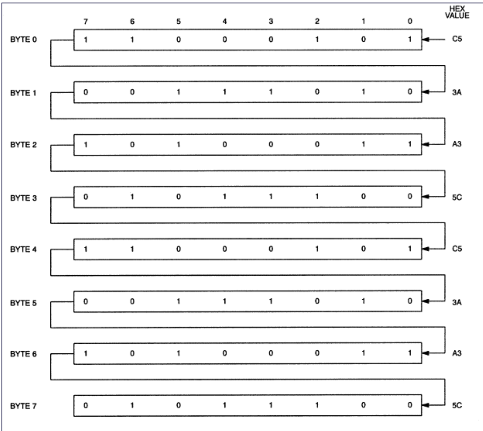
Figure 4. Time chip comparison register definition.
