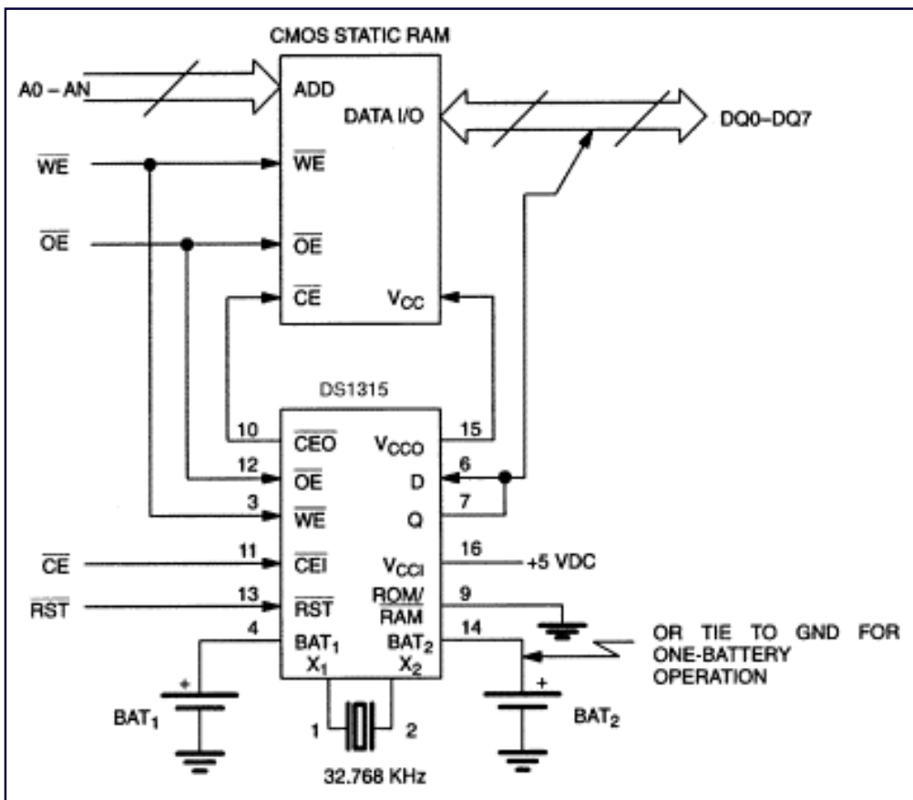
Figure 1. RAM/Time chip interface.
