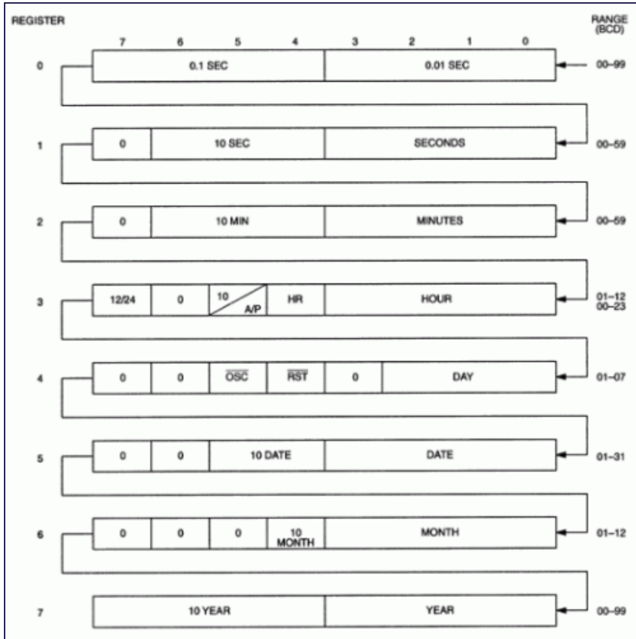
Figure 5. Time chip register definition.
