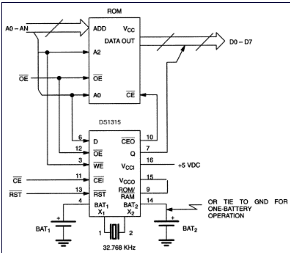
Figure 2. ROM/Time chip interface.
