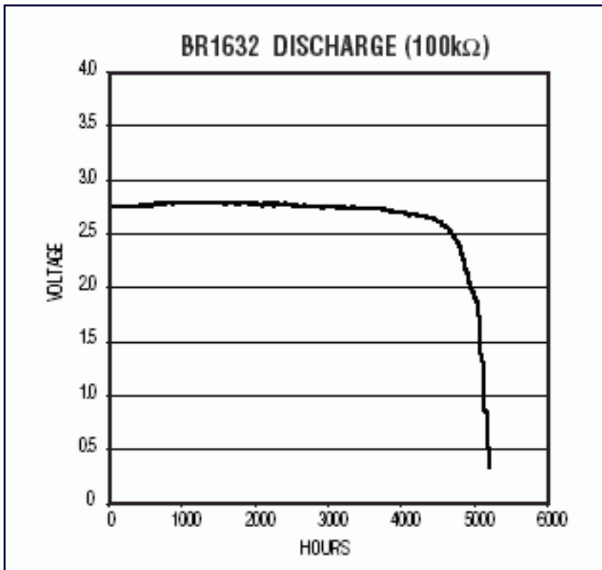
Figure 2. The output voltage remains constant during discharge.
