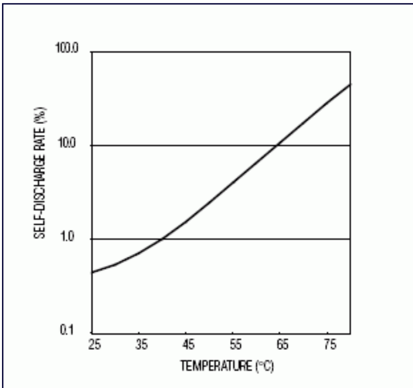
Figure 4. The self-discharge rate increases as temperature increases.
