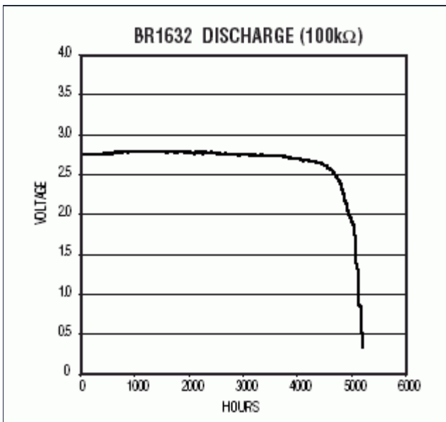
Figure 2. The output voltage remains constant during discharge.
