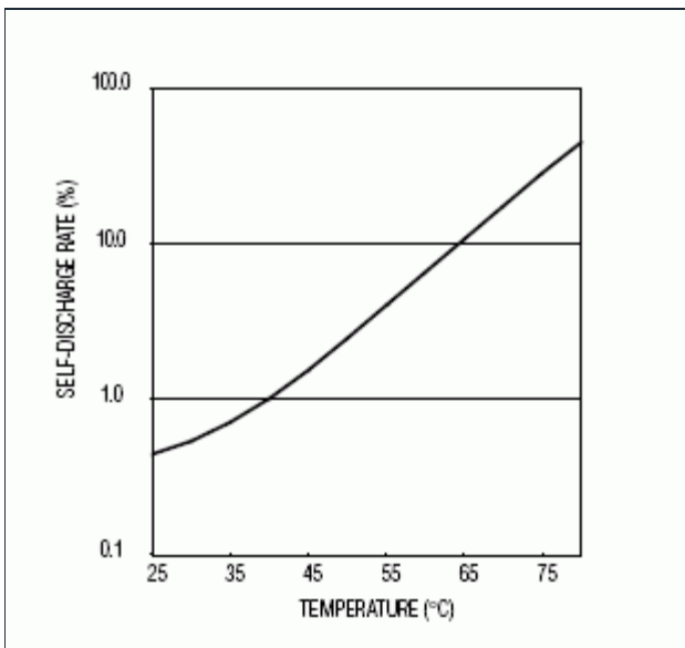
Figure 4. The self-discharge rate increases as temperature increases.
