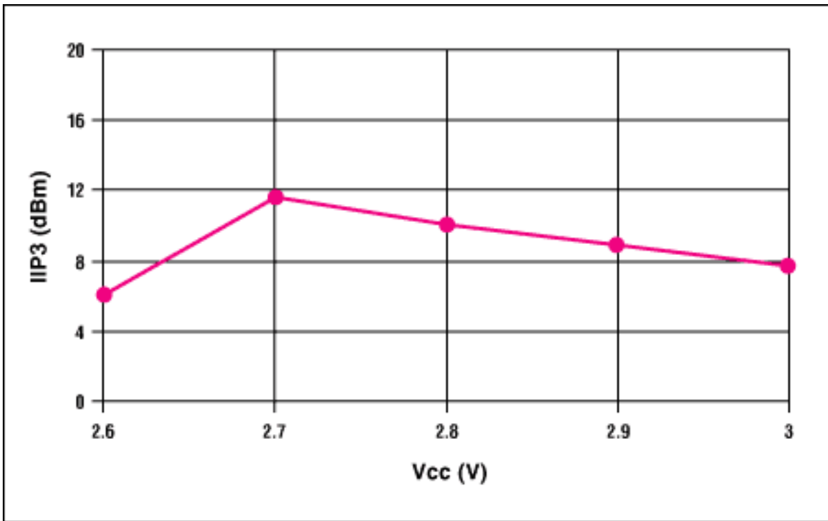
Figure 2. Mixer IIP3 versus V_{CC} .
