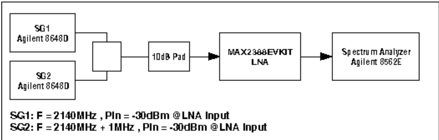
Figure 3. MAX2388 LNA IIP3 measurement.
