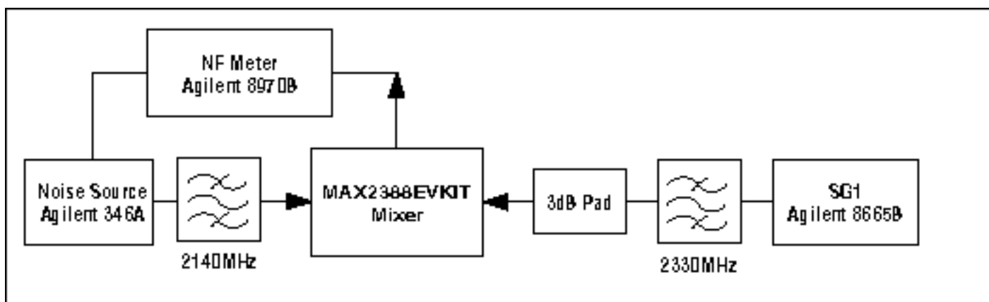
Figure 6. MAX2388 mixer NF measurement.
