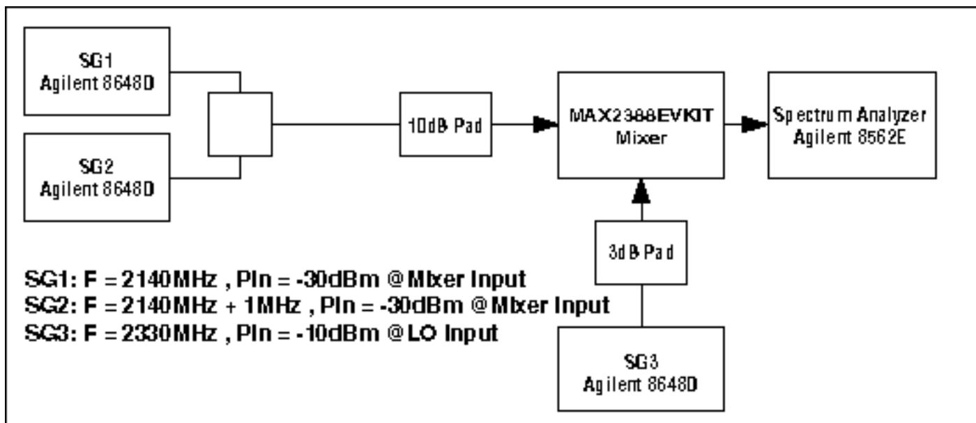
Figure 4. MAX2388 mixer IIP3 measurement.
