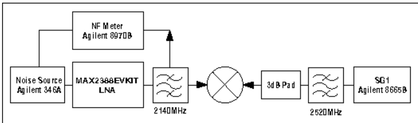
Figure 5. MAX2388 LNA NF measurement.
