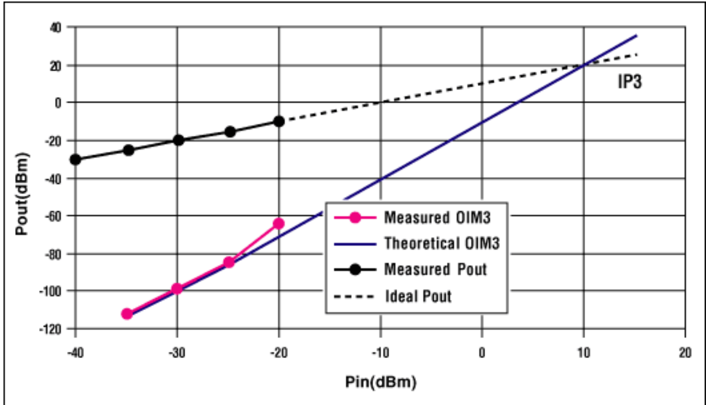
Figure 1. MAX2388 mixer IIM3 versus pin.
