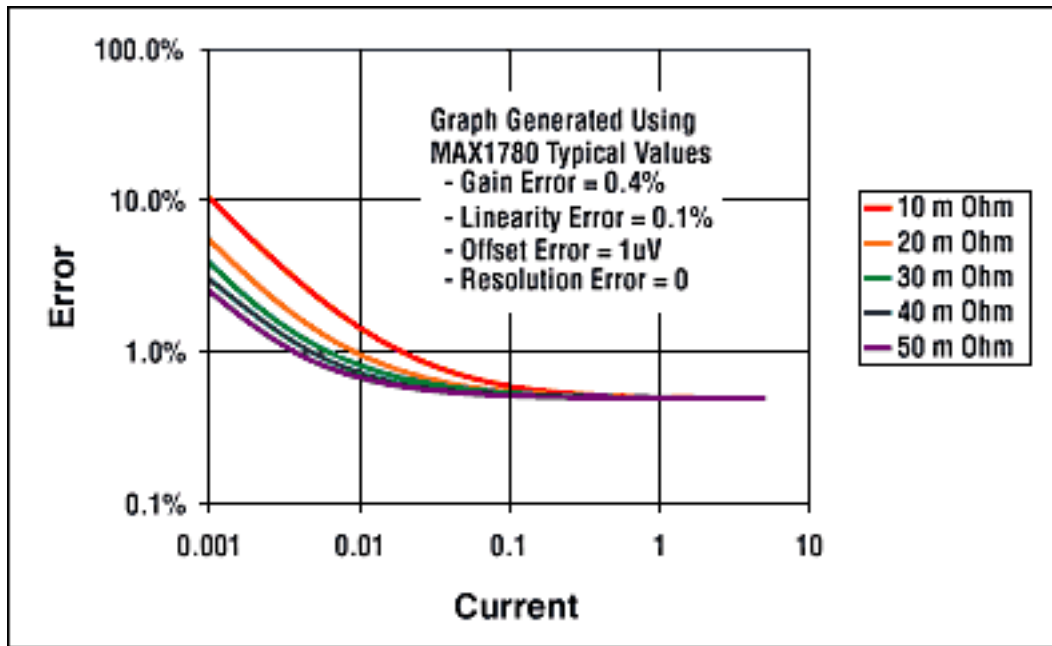
Figure 3. Coulomb-counter accuracy as a function of current and R_{\text{SENSE}} .
