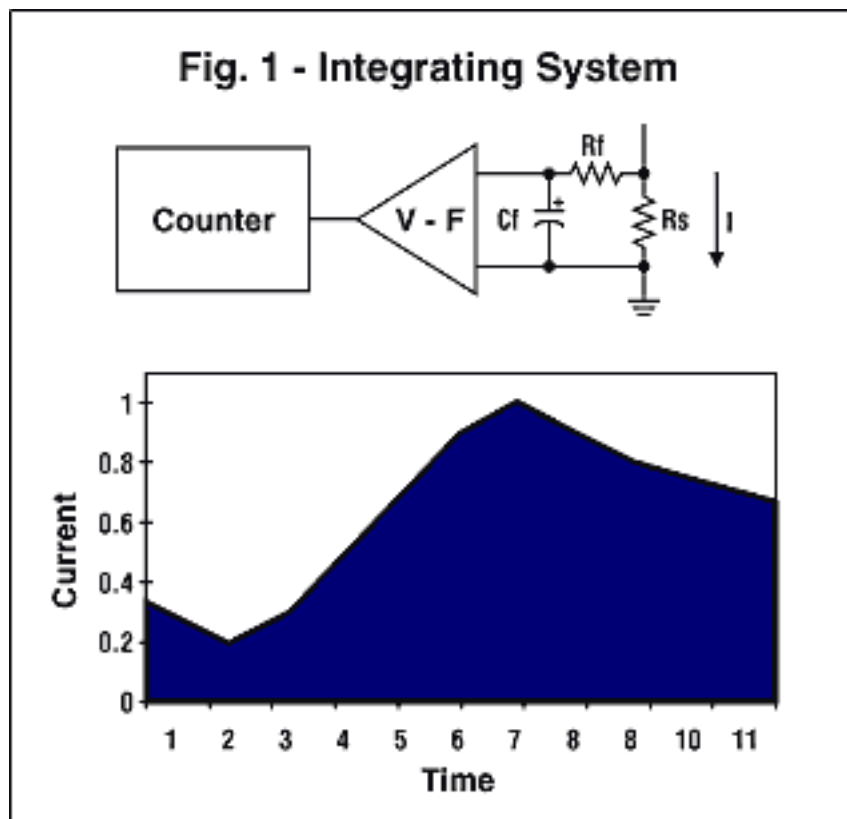
Figure 1. Integrating system.
