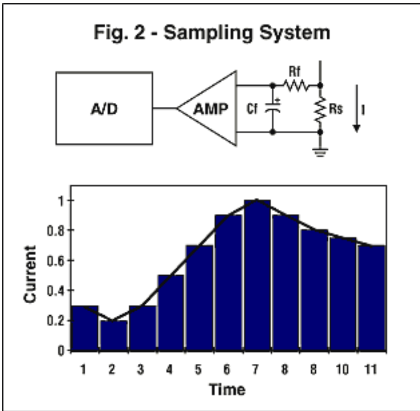
Figure 2. Sampling system.
