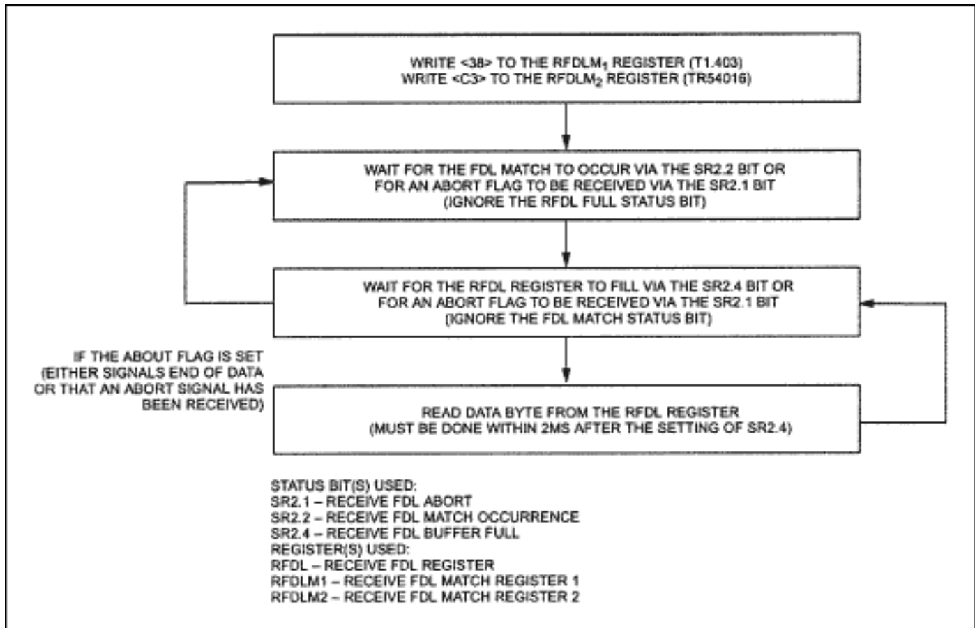
Figure 1. Receive FDL decoding.
