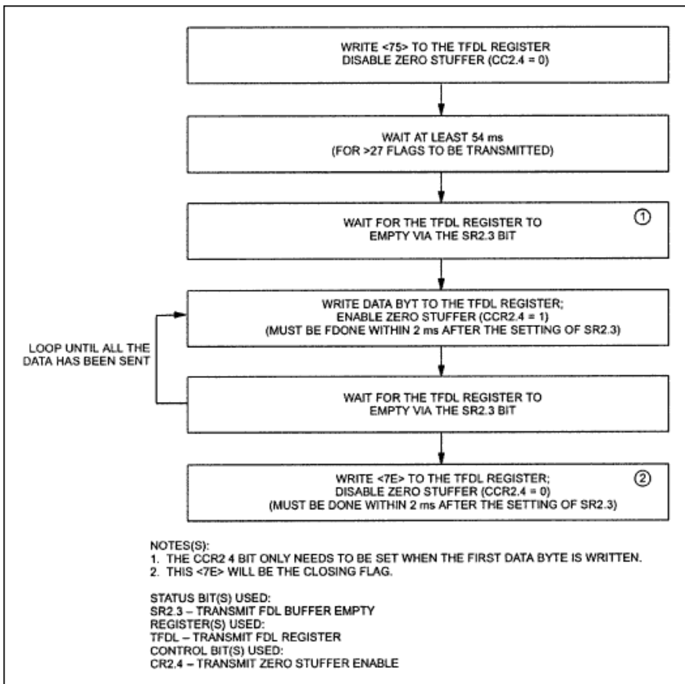
Figure 3. Transmit FDL coding.
