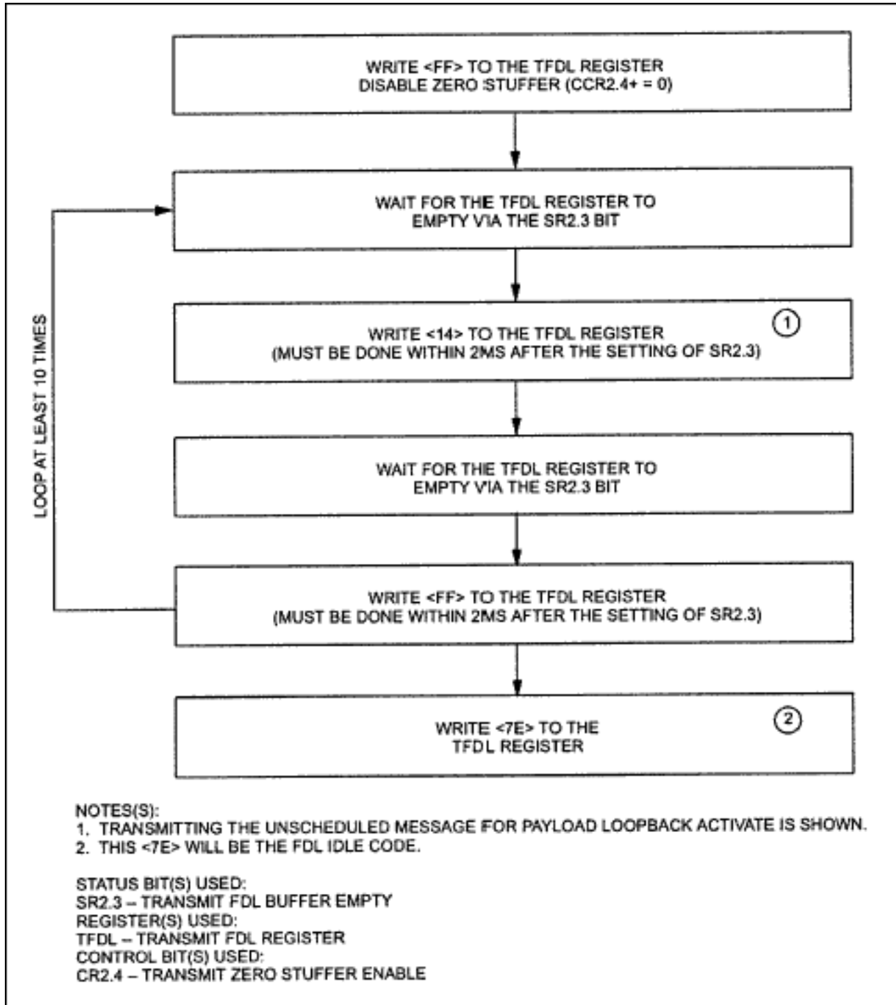
Figure 2. Transmit T1.403 unscheduled message.
