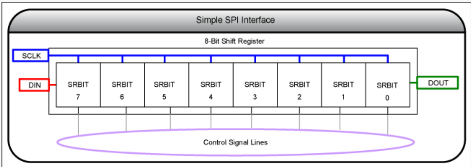
Figure 1. Simple representation of an 8-bit SPI interface.
