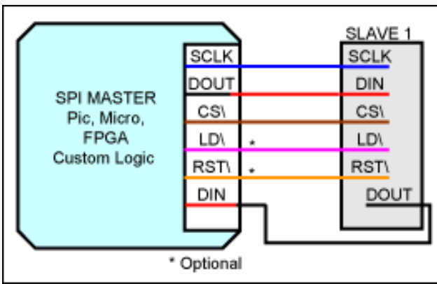
Figure 4. Single master/slave SPI interface.
