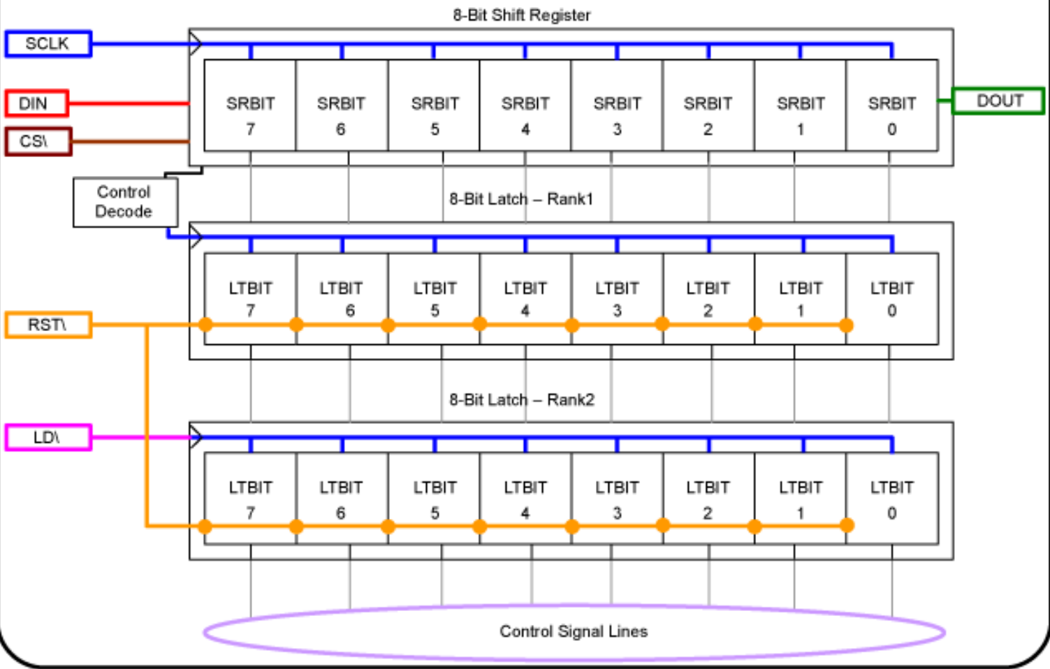
Figure 2. Simple example of an 8-bit-word, dual-rank SPI interface.
