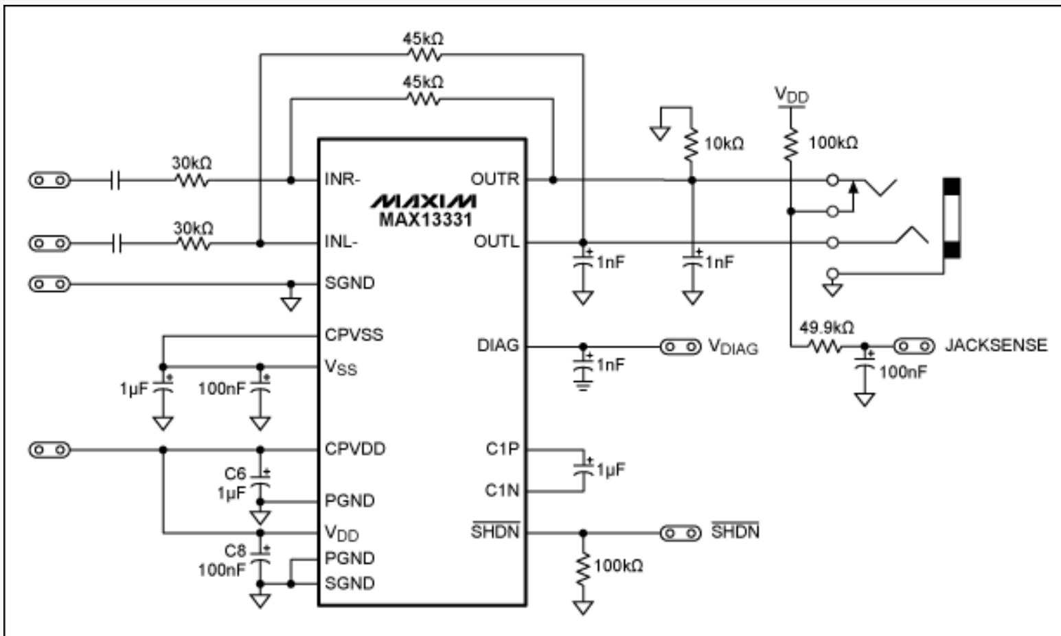
Figure 2. Schematic diagram of MAX13331 with discrete jack-sensing circuit.
