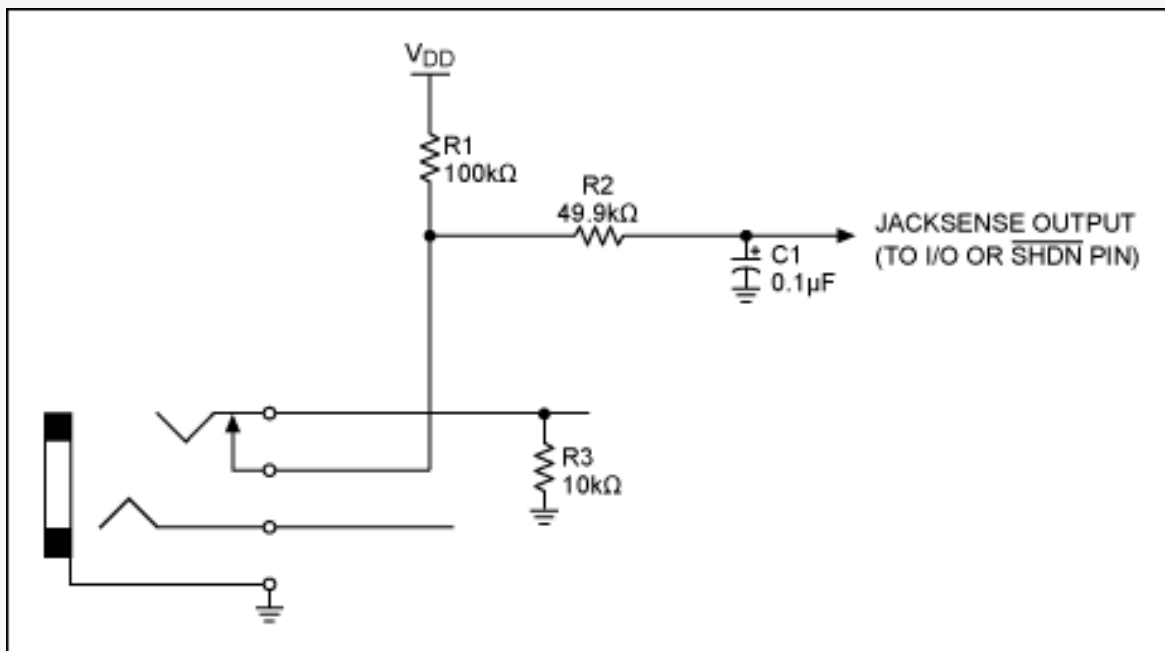
Figure 1. Jack-sensing circuit.
