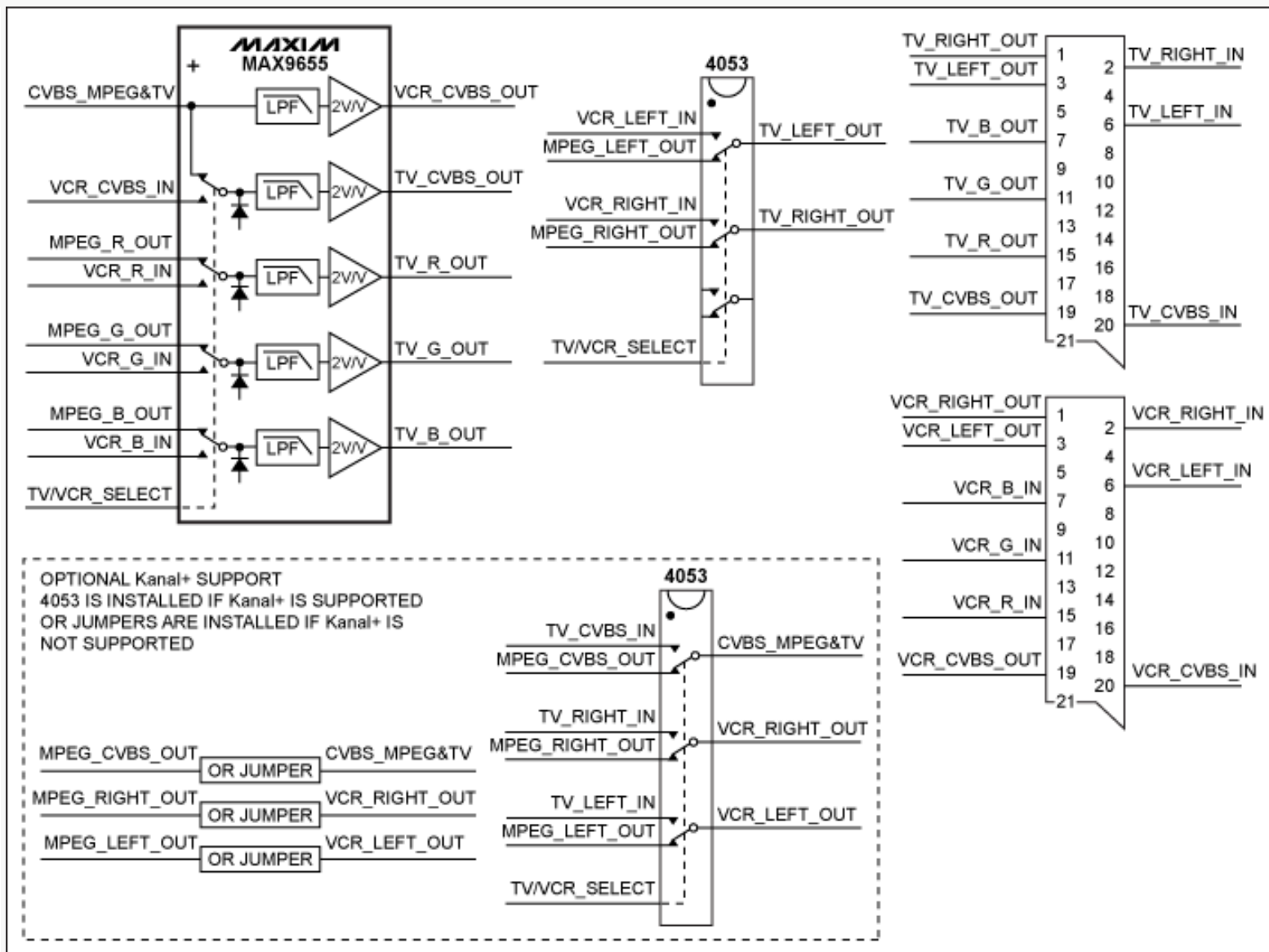
Figure 2. Optional Kanal+ support is provided by adding a second 4053 multiplexer to the MAX9655 design in Figure 1.
