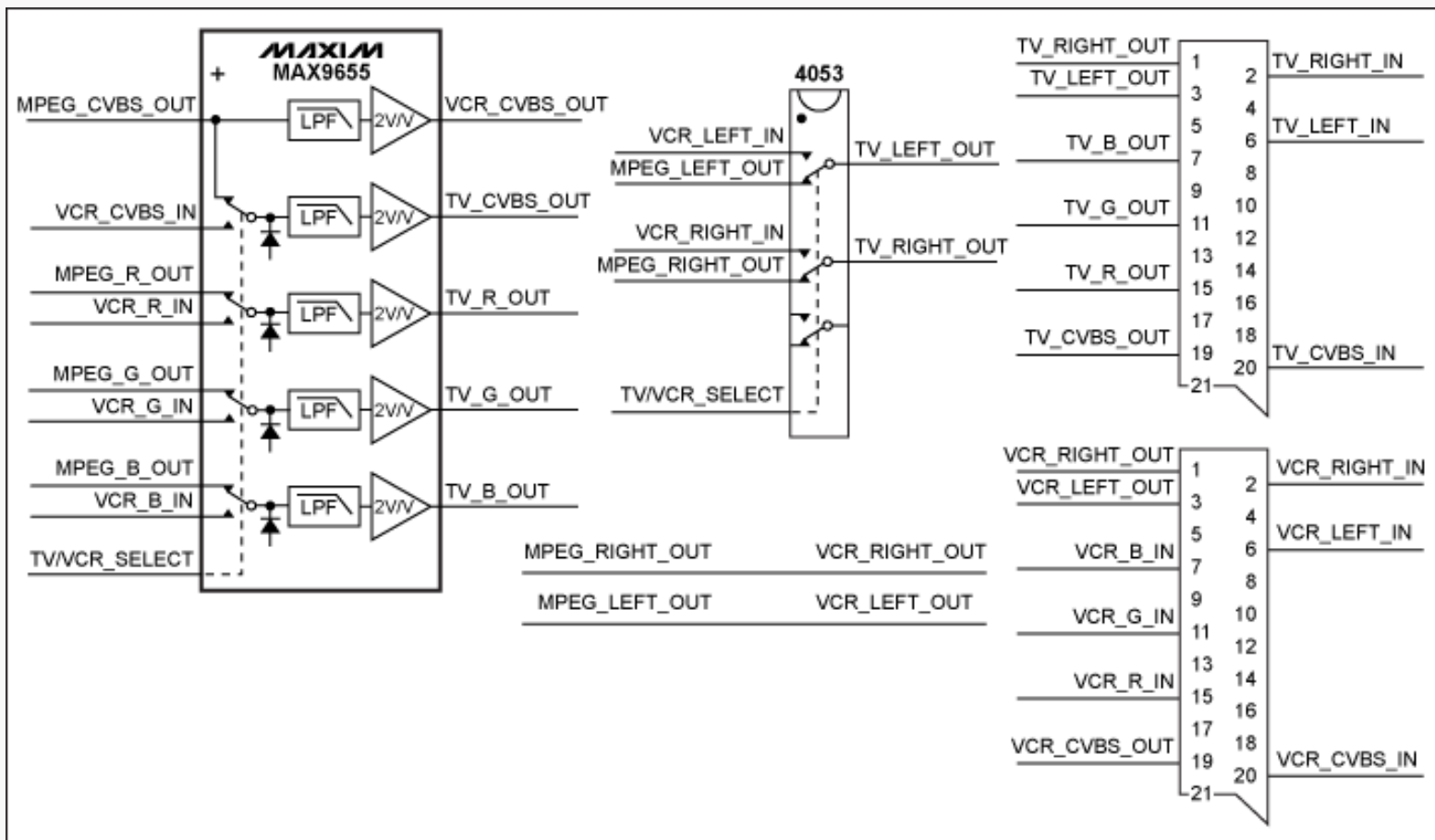
Figure 1. Basic block diagram uses a MAX9655 and a 4053 for dual SCART solution.
