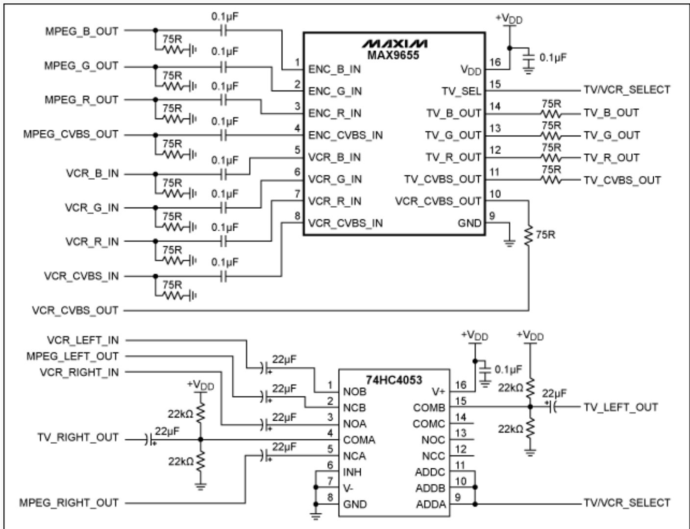
Figure 3. Schematics for the basic dual SCART switch in Figure 1.
