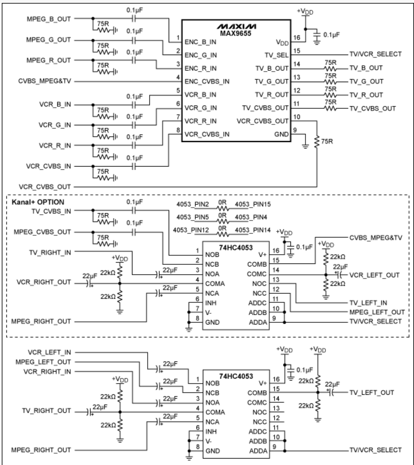
Figure 4. Schematics for the dual SCART switch with Kanal+ support in Figure 2.
