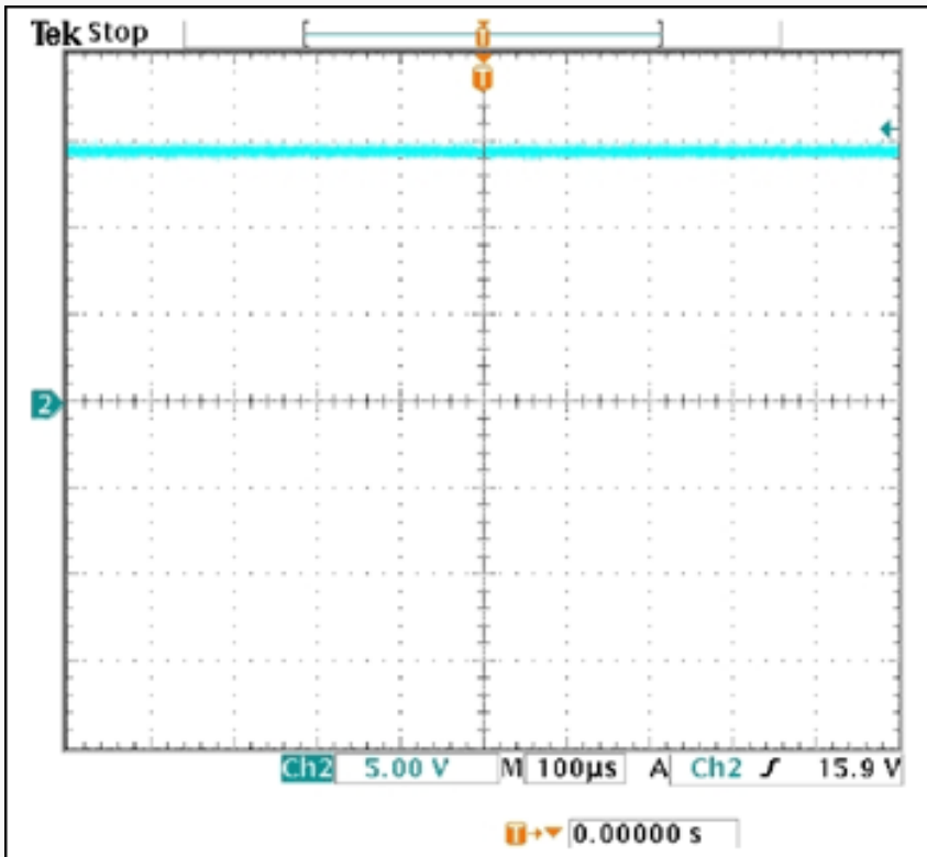
Figure 6. LED voltage.
