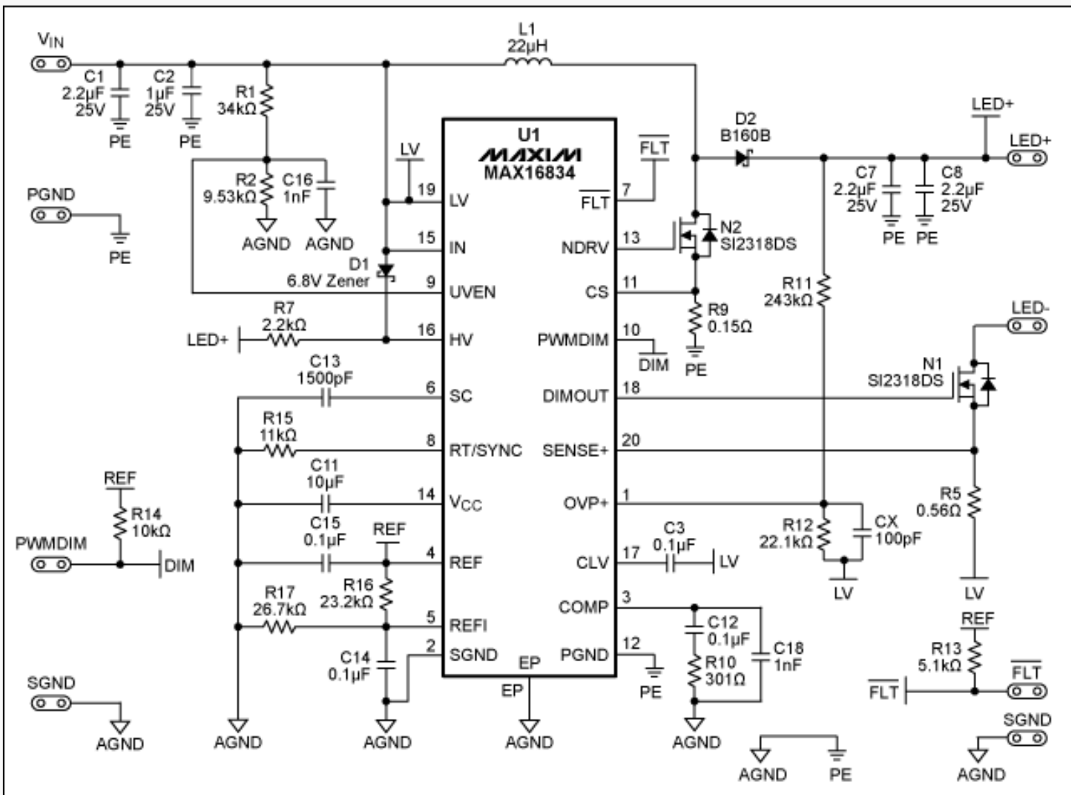
Figure 2. Schematic of the LED driver.
