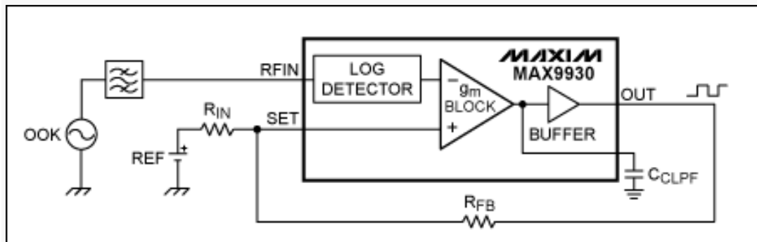
Figure 3. Circuit showing the MAX9930 RF-detecting controller in an OOK application.
