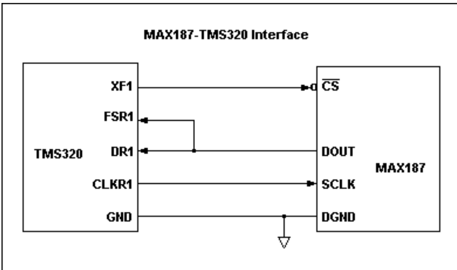
Figure 1. MAX187-TMS320 interface.
