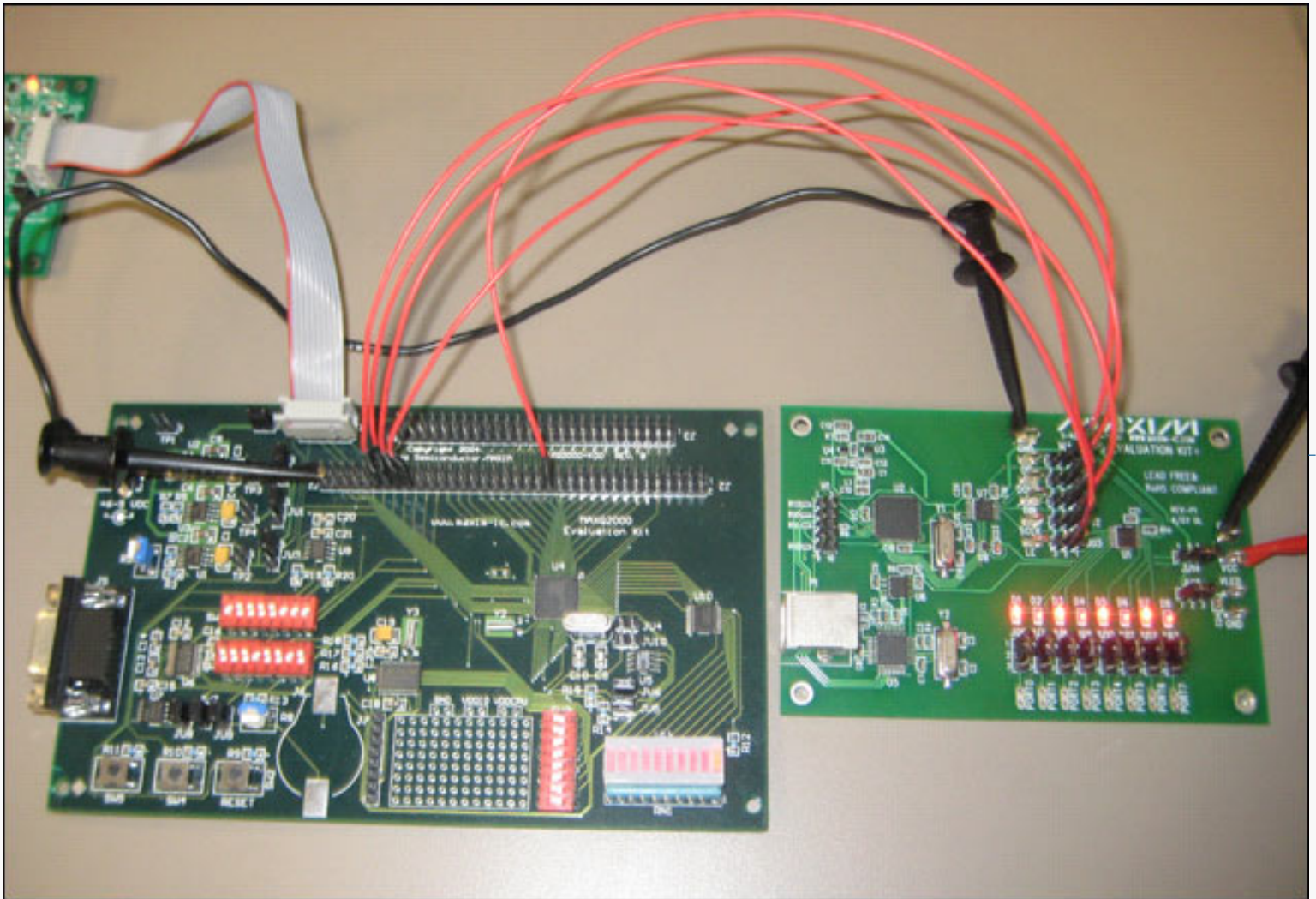
Figure 3. MAXQ2000 EV kit and MAX6970 EV kit setup.
