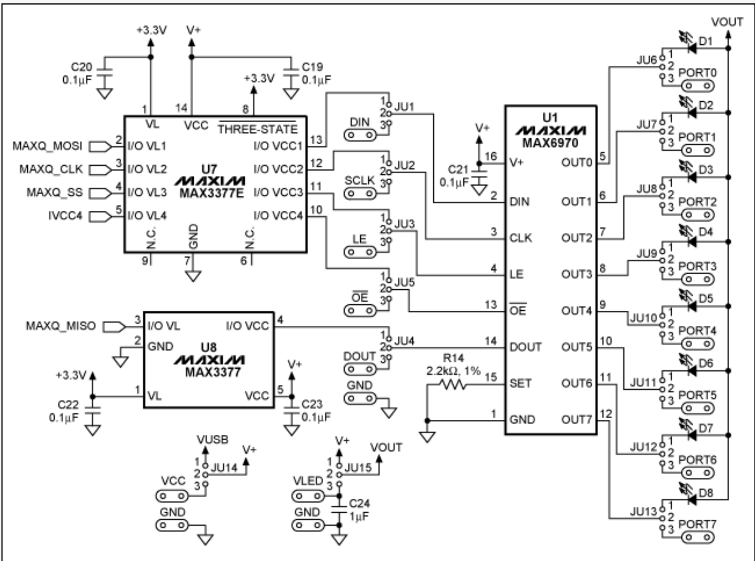
Figure 1. MAX6970EVKIT schematic.
