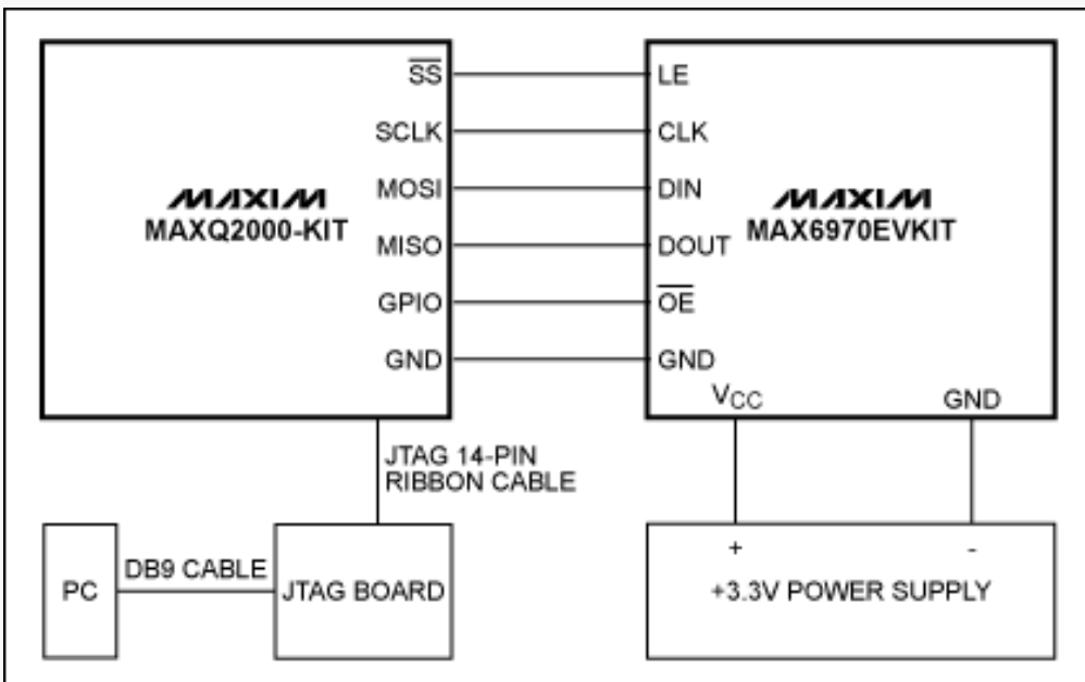
Figure 2. Hardware configuration block diagram.
