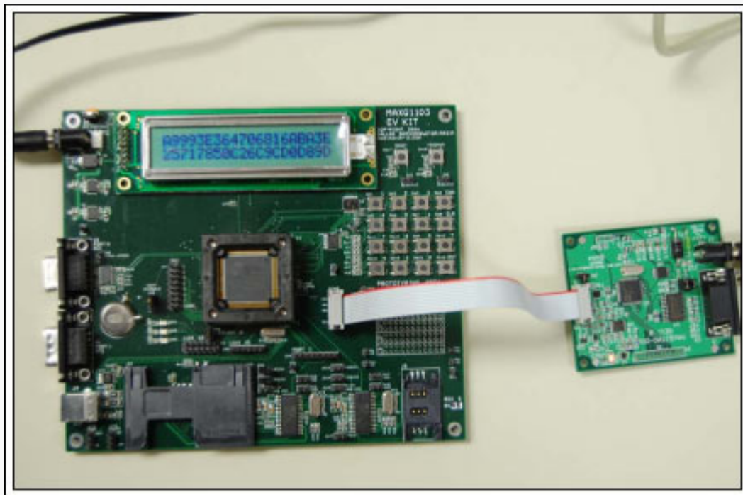
Figure 1. MAXQ1103 EV kit with JTAG board.
