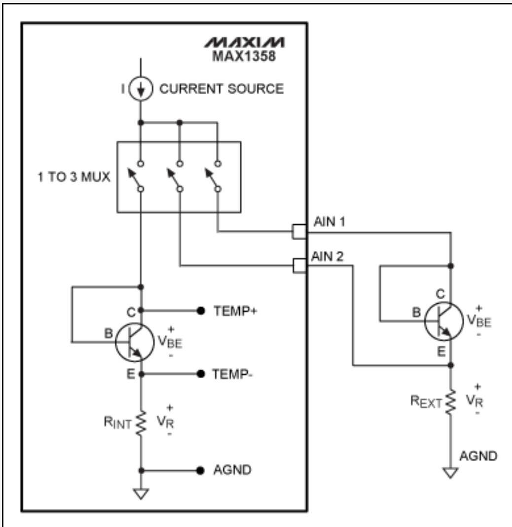
Figure 1. MAX1358 internal/external temperature measurement circuit.
