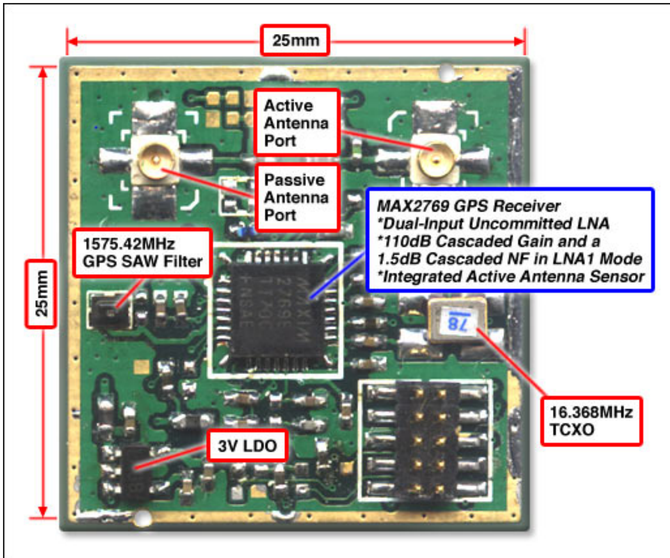
Figure 1. GPS reference design features the MAX2769 .
