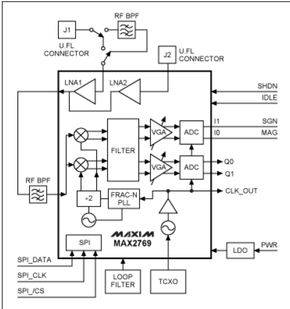
Figure 2. Block diagram for the GPS reference design.
