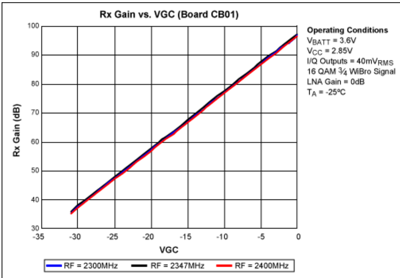
Figure 6. Receive gain characteristic across the 2.3GHz to 2.4GHz band. Gain variation over frequency is less than 0.2dB. Gain-control range, not including LNA gain steps, is 62dB, approximately 2dB per gain step.
