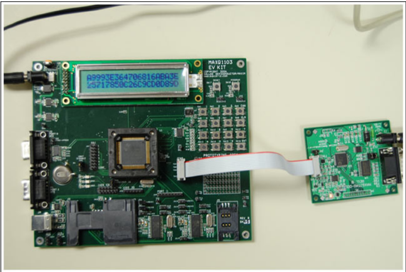
Figure 1. MAXQ1103 EV kit.
