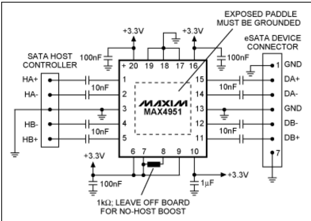
Figure 5. This laptop/desktop design incorporates the MAX4951 to boost SATA signals to eSATA levels.
