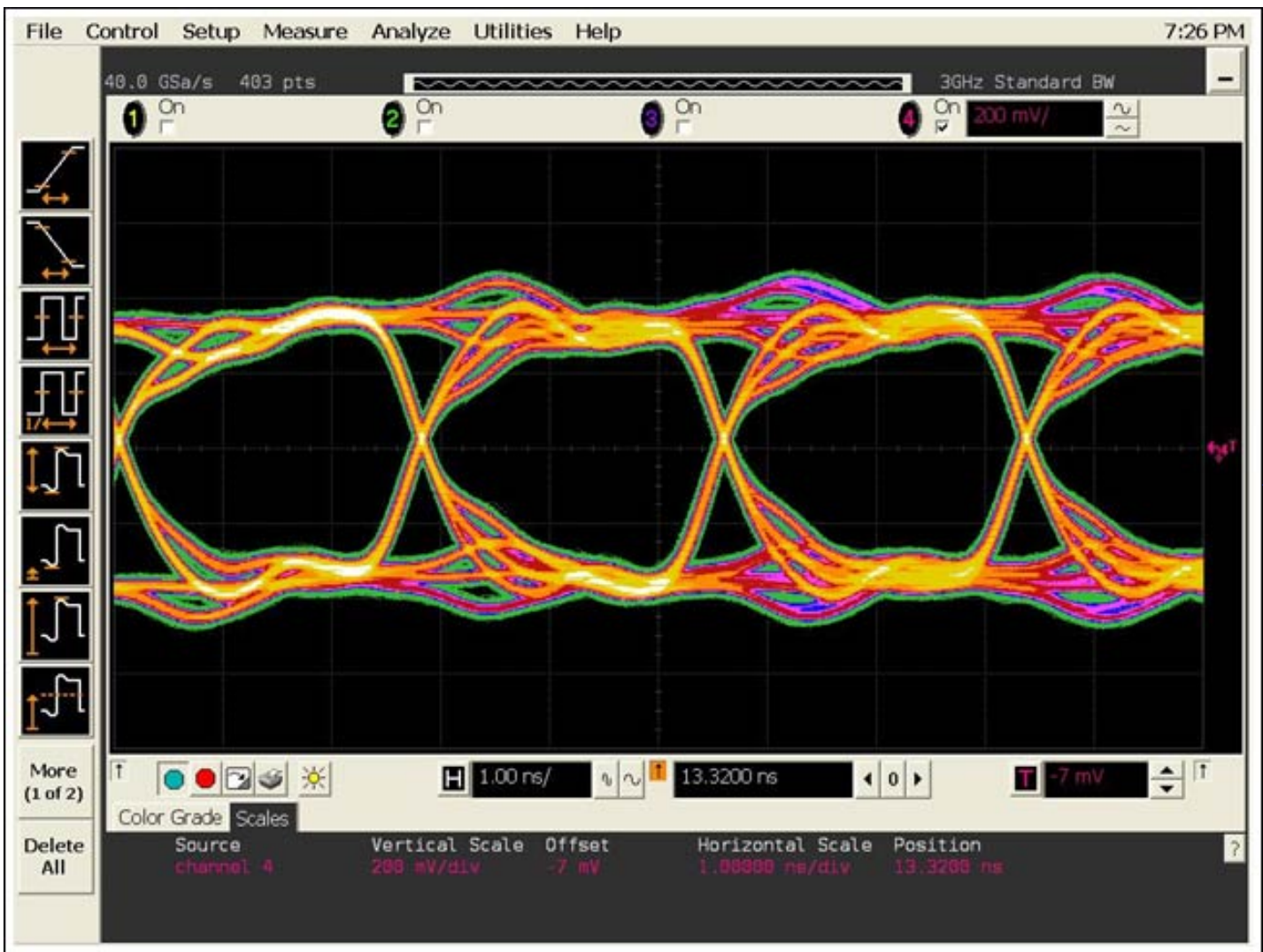
Figure 6. Permanent PRBS mode—eye diagram, JAE connector 0.5m.
