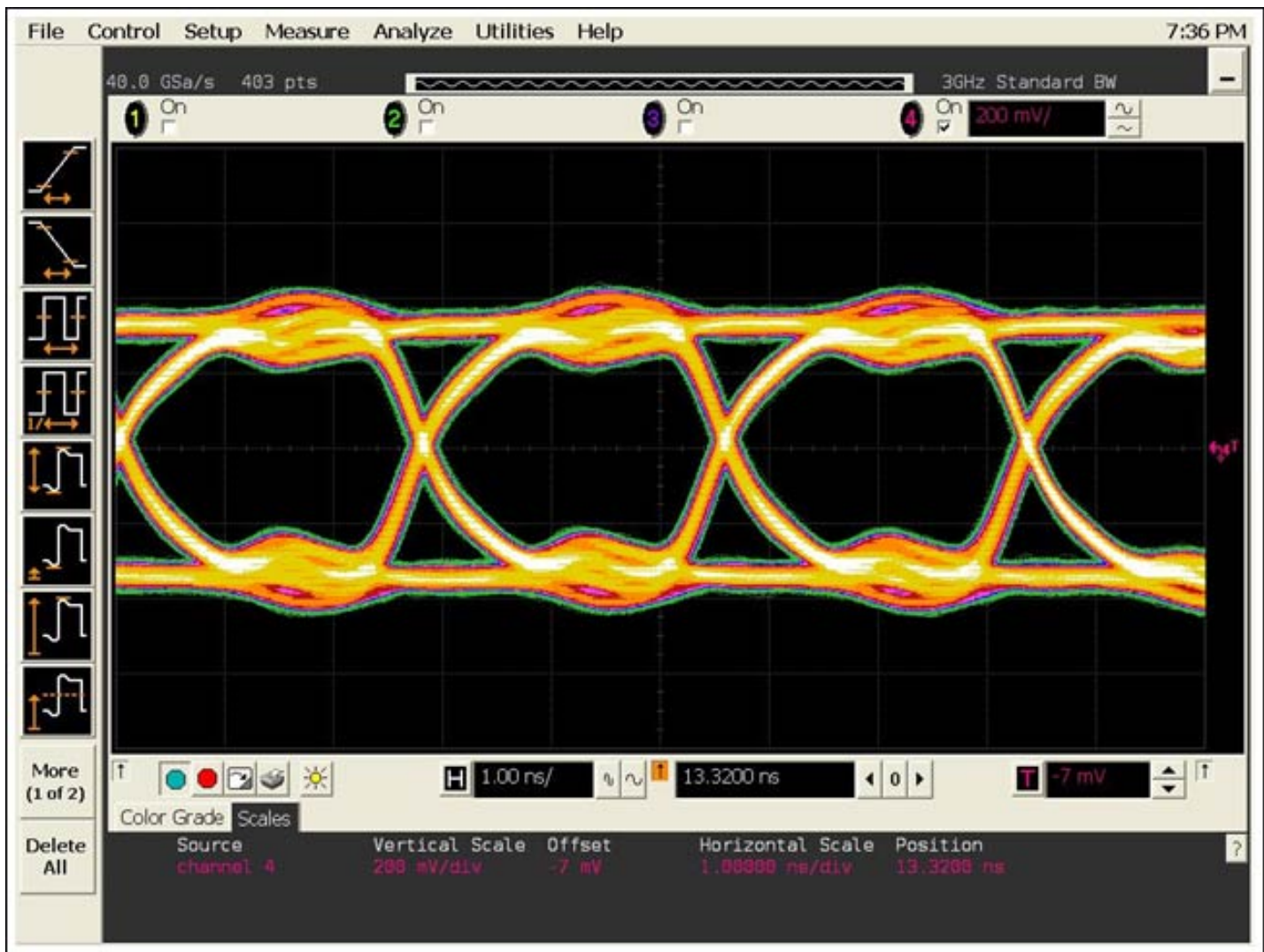
Figure 7. Permanent PRBS mode—eye diagram, JAE connector 2m.
