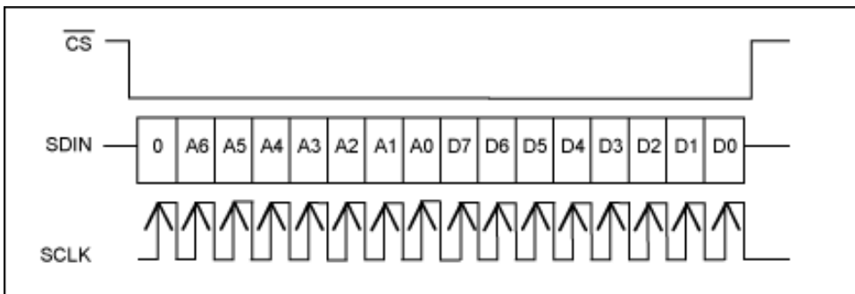
Figure 1. Write operation.
