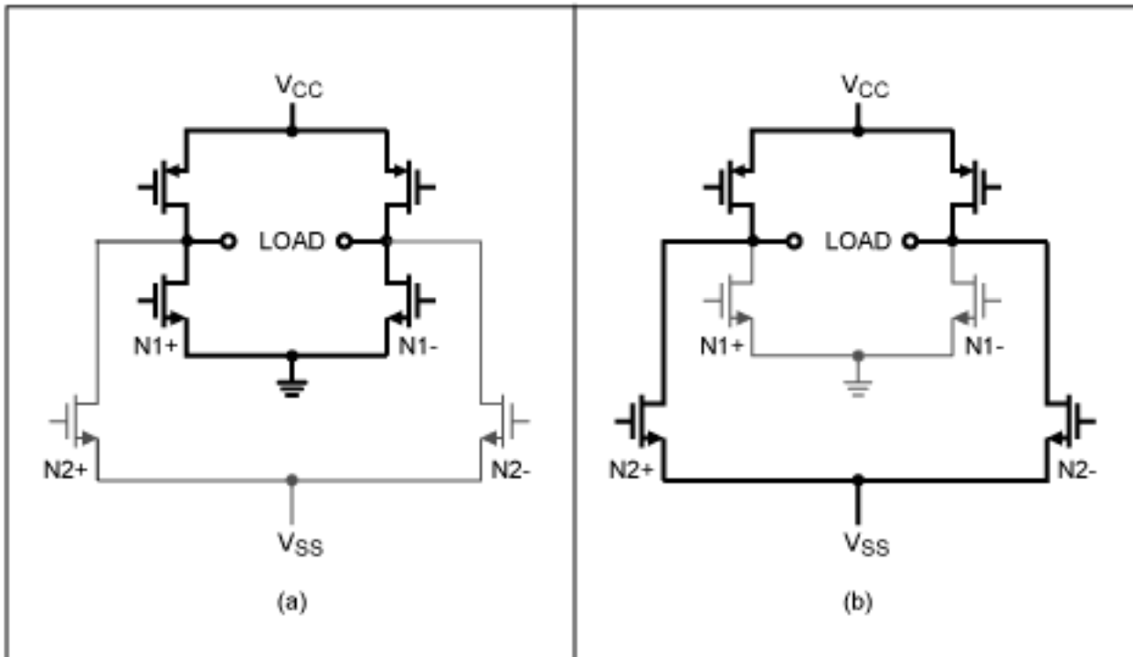
Figure 1a and b. MAX9788 Class G output stage operating from the low supply (a), and from the high supply (b).
