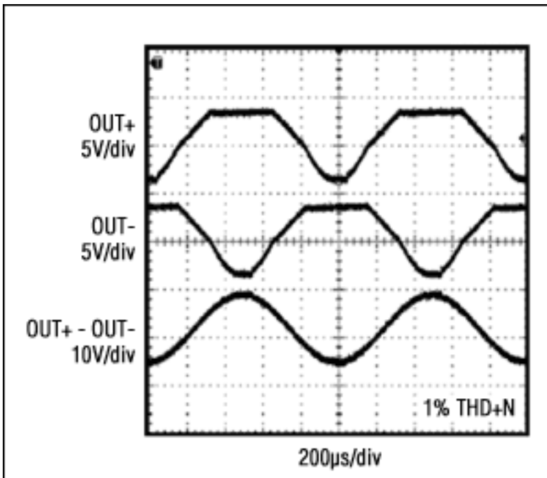
Figure 2. A Class G output waveform generated with the MAX9788 amplifier.
