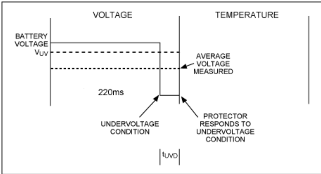
Figure 2. Conditions for minimum t_{UV D} . In this example, the battery voltage is above V_{UV} for the majority of the measurement window, but it then falls far enough below the undervoltage threshold to bring the average voltage measured during the 220ms window below V_{UV} .
