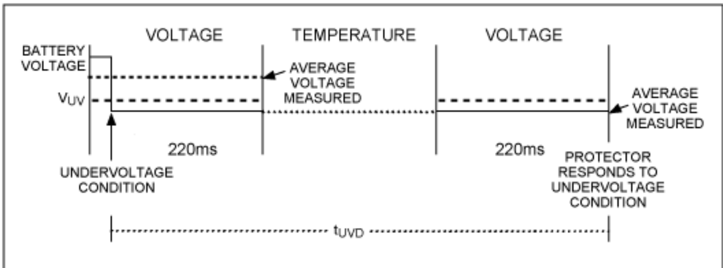
Figure 3. Conditions for maximum t_{UV D} . In this example, the battery voltage is far enough above V_{UV} that even when the voltage falls below the undervoltage threshold, the average voltage for the 220ms window remains above V_{UV} . Thus, an undervoltage condition is not registered until the next voltage measurement window.
